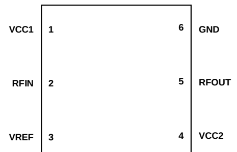
Figure 2. CX65102 Pinout – 6-Pin LCC Package Top View
