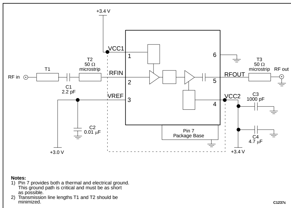
Figure 9. Evaluation Board Schematic, 1700 MHz to 2200 MHz
