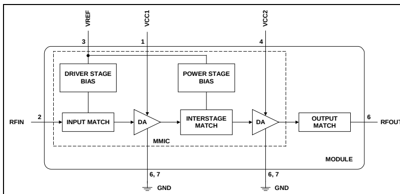
Figure 1. CX65102 Functional Block Diagram
