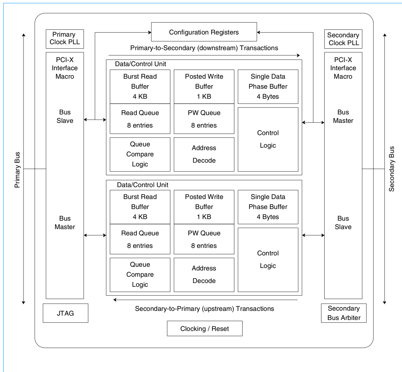
Figure 2-1. Block Diagram
