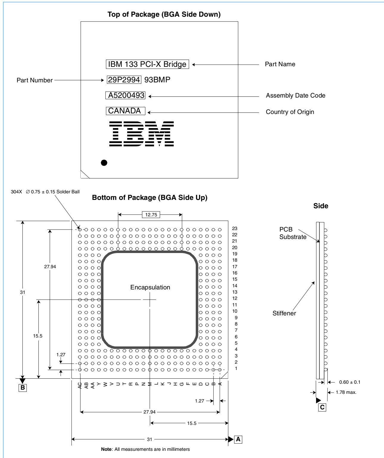
Figure 11-1. Package Diagram 31 x 31 mm 304-lead H-PBGA Package
