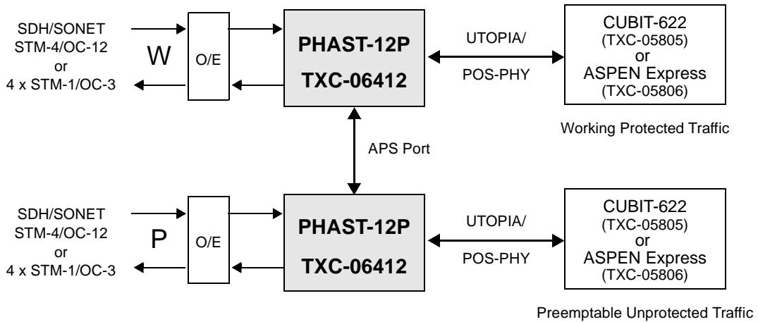
Figure 52. STM-4/OC-12 or 4 x STM-1/OC-3 1+1, 1:1 APS Line Protection
