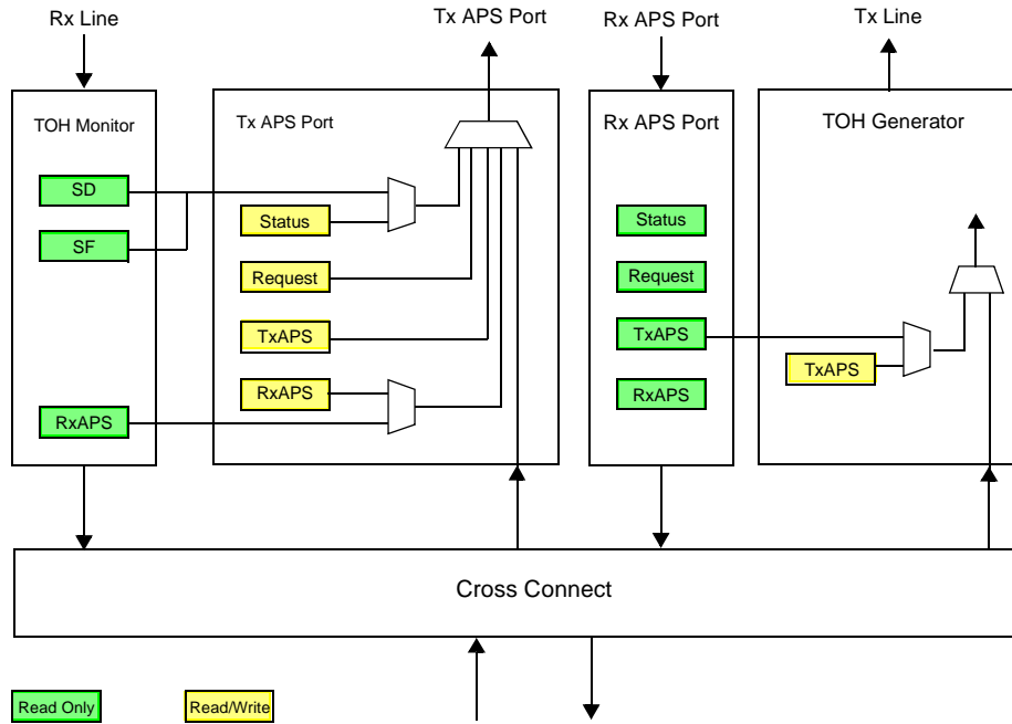
Figure 24. APS Port Architecture
