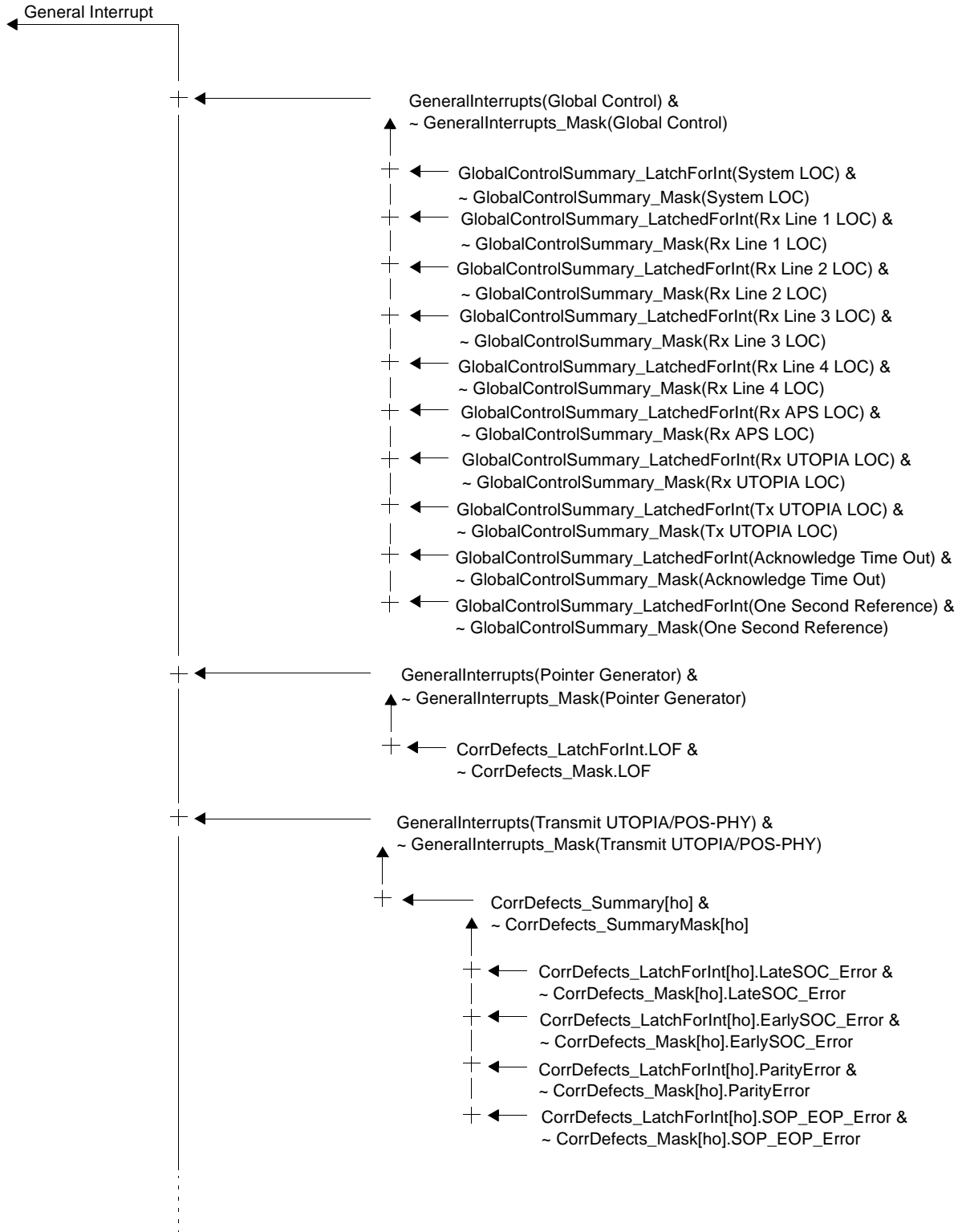
Figure 45. General Interrupt Tree (part 1)
