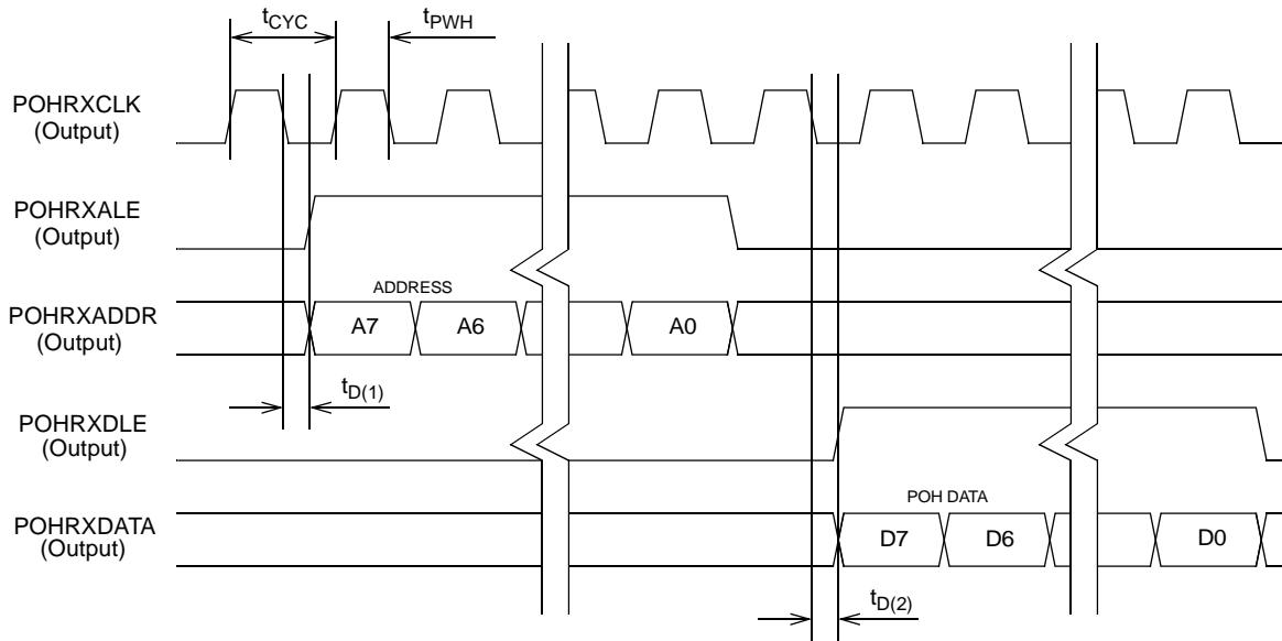
Figure 7. RX High Order POH Byte Interface
