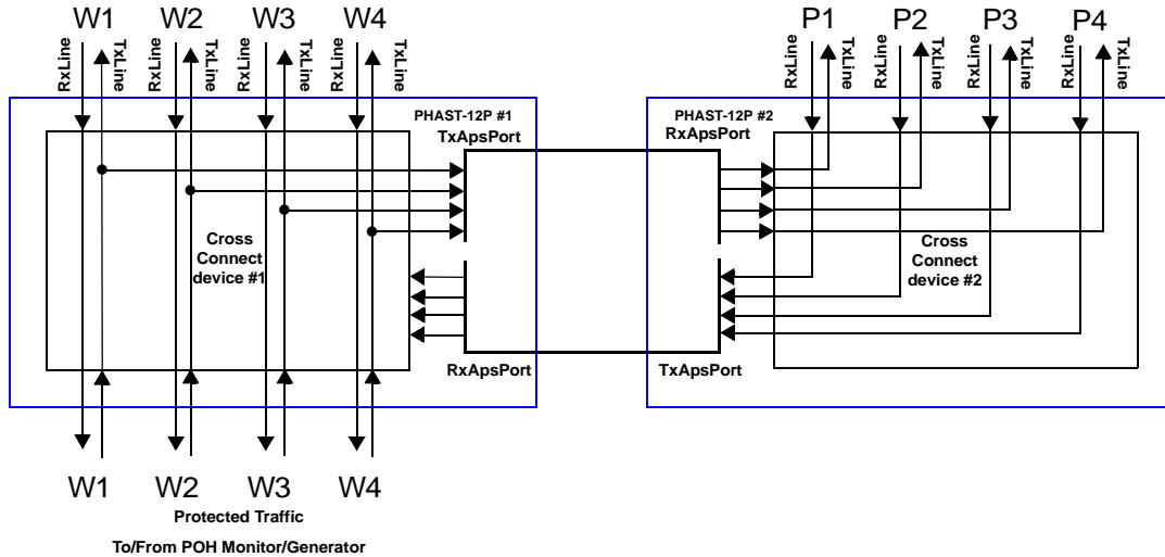
Figure 27. STM-1/OC-3, 1+1 APS Idle State
