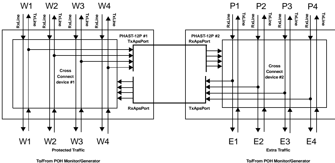
Figure 29. STM-1/OC-3, 1:1 APS Idle State
