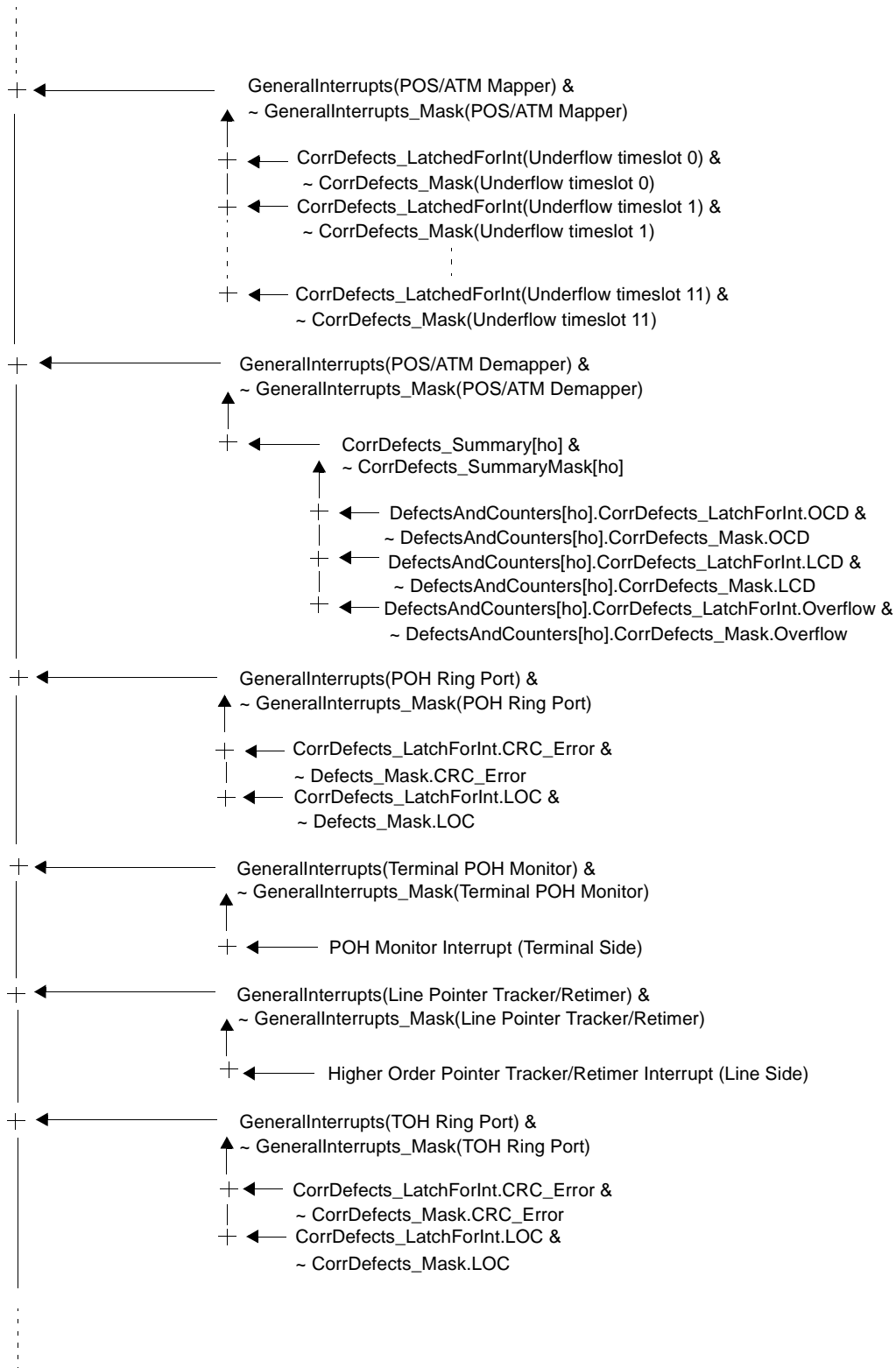
Figure 46. General Interrupt Tree (part 2)
