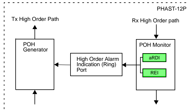
Figure 37. Internal High Order Alarm Indication (Ring) Port Interface
