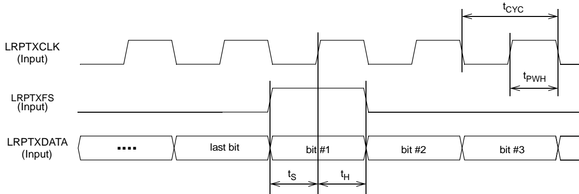
Figure 10. TX Line Ring Port Interface
