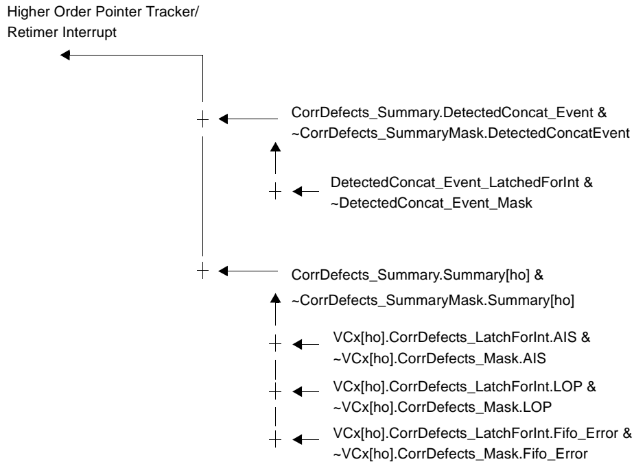
Figure 40. High Order Point Tracker Retimer Interrupt Tree
