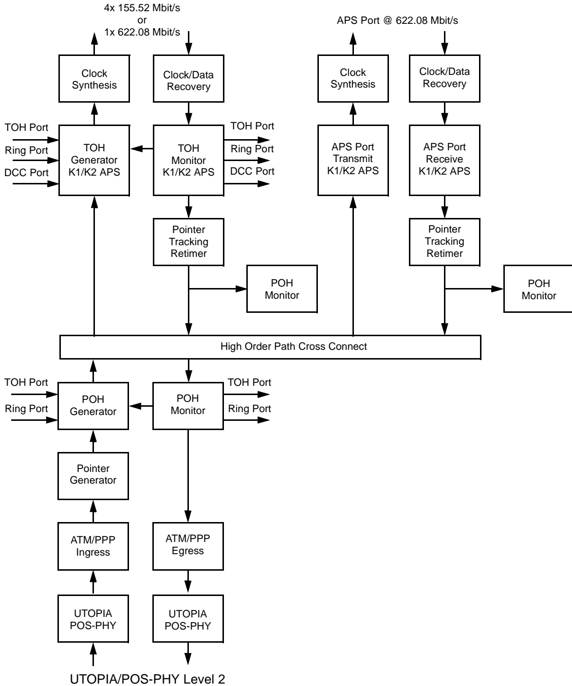
Figure 2. PHAST-12P TXC-06412 Block Diagram
