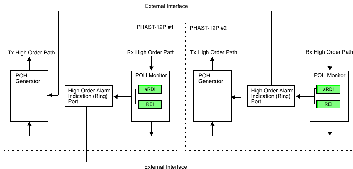
Figure 38. External High Order Alarm Indication (Ring) Port Interface
