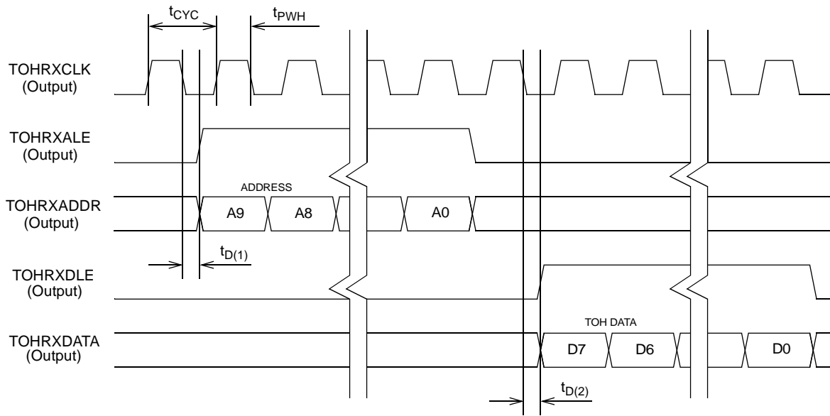
Figure 5. RX TOH Byte Interface
