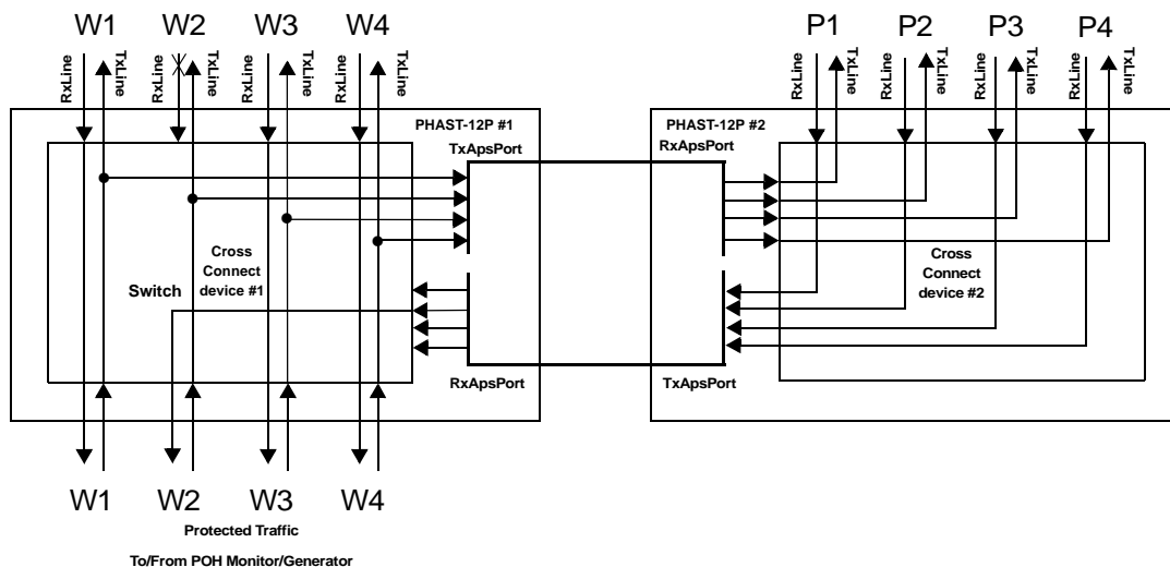
Figure 28. STM-1/OC-3, 1+1 APS Switch State
