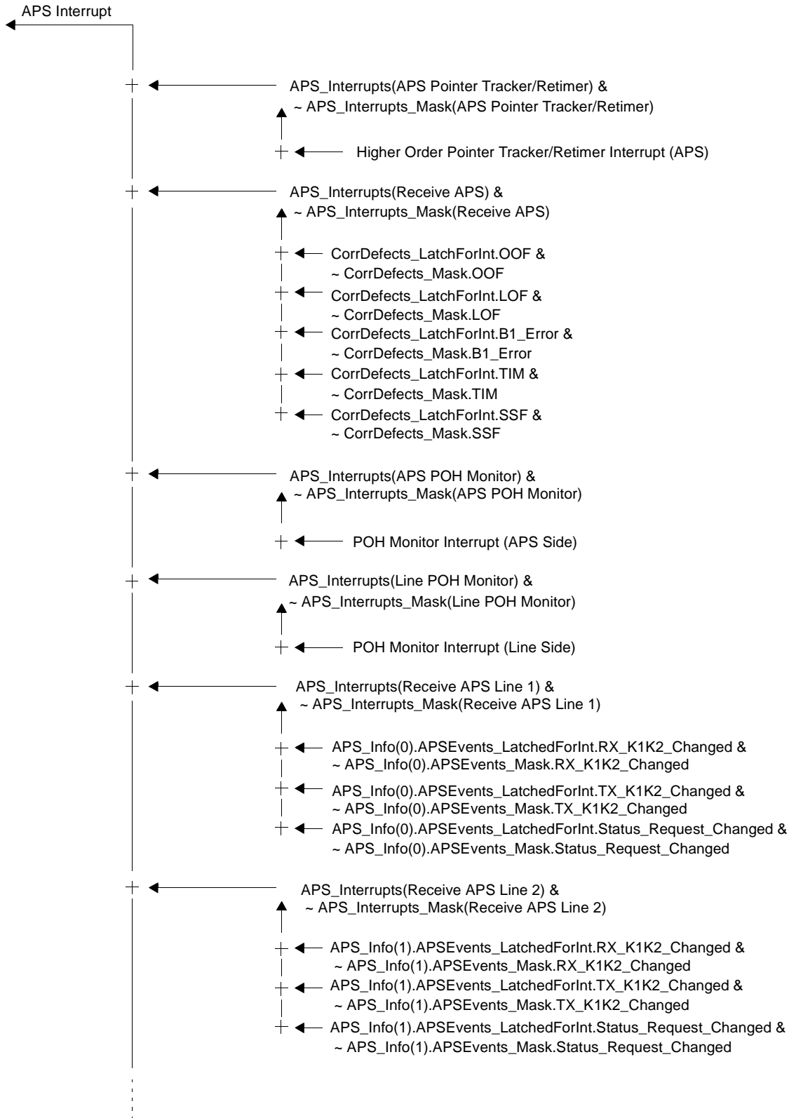
Figure 43. APS Interrupt Tree (part 1)
