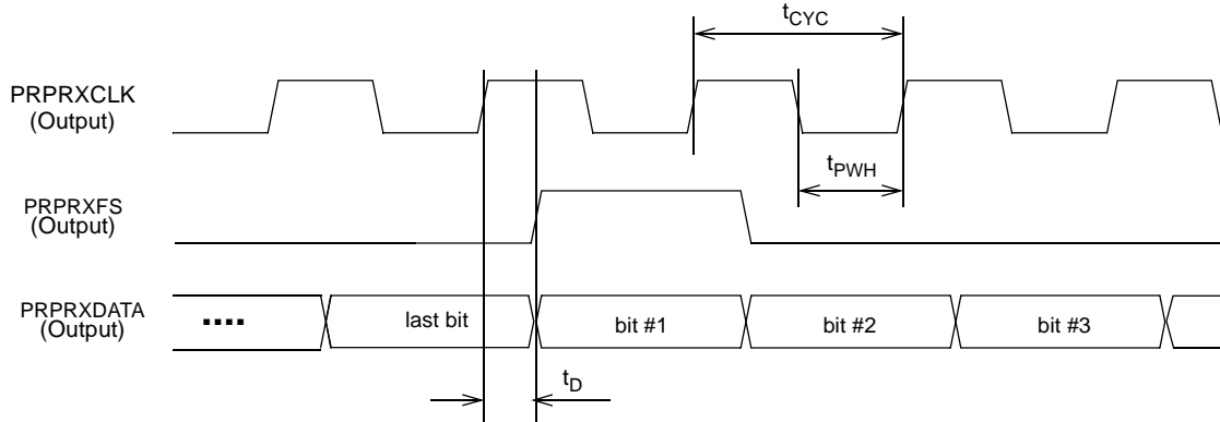
Figure 11. RX Path Alarm Indication Port Interface
