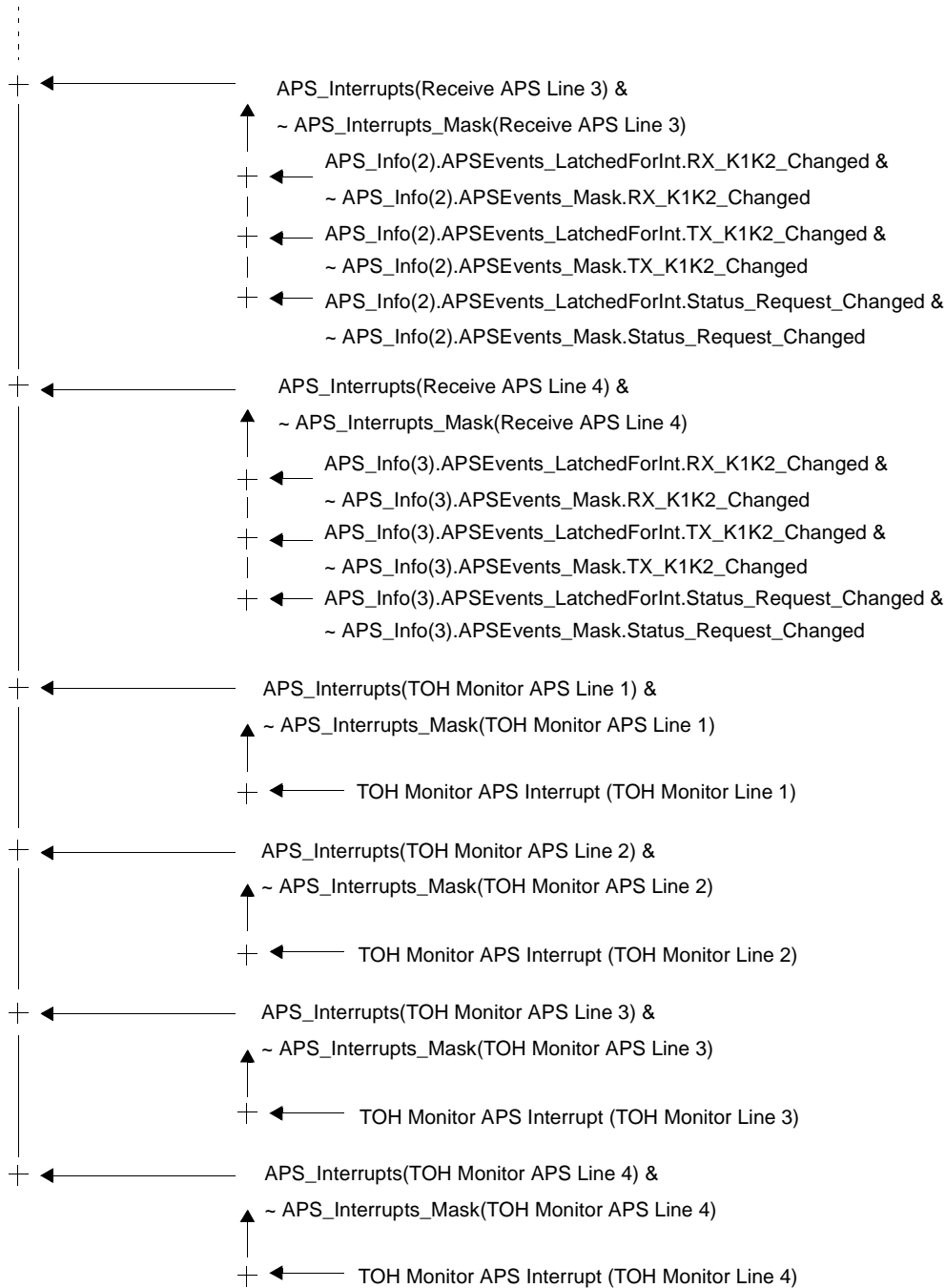
Figure 44. APS Interrupt Tree (part 2)
