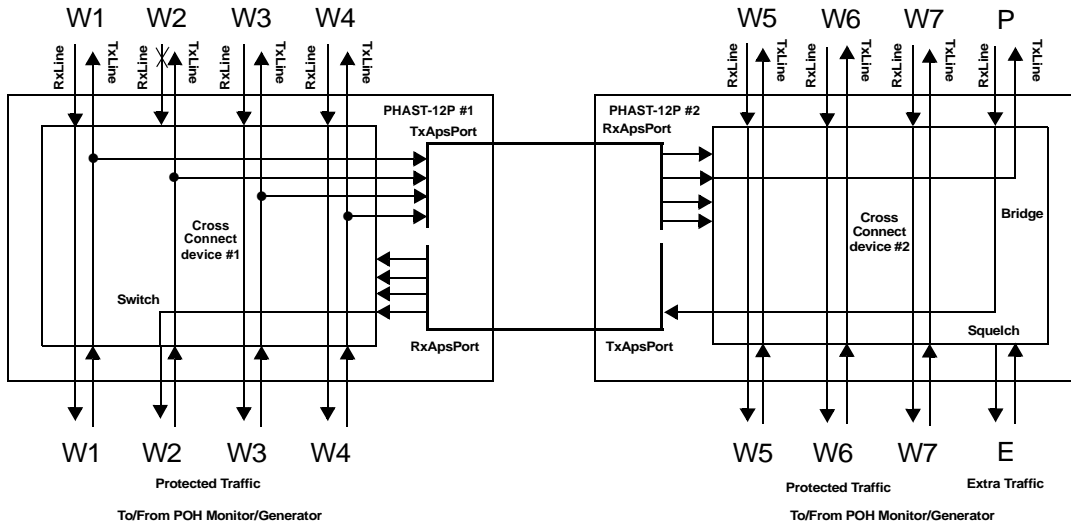
Figure 32. STM-1/OC-3, 1:7 APS Switch State
