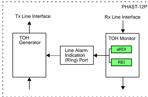
Figure 35. Internal Line Alarm Indication (Ring) Port Interface
