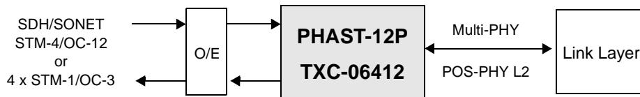
Figure 51. STM-4/OC-12 or 4 x STM-1/OC-3 IP (PPP) DSLAM Network Card
