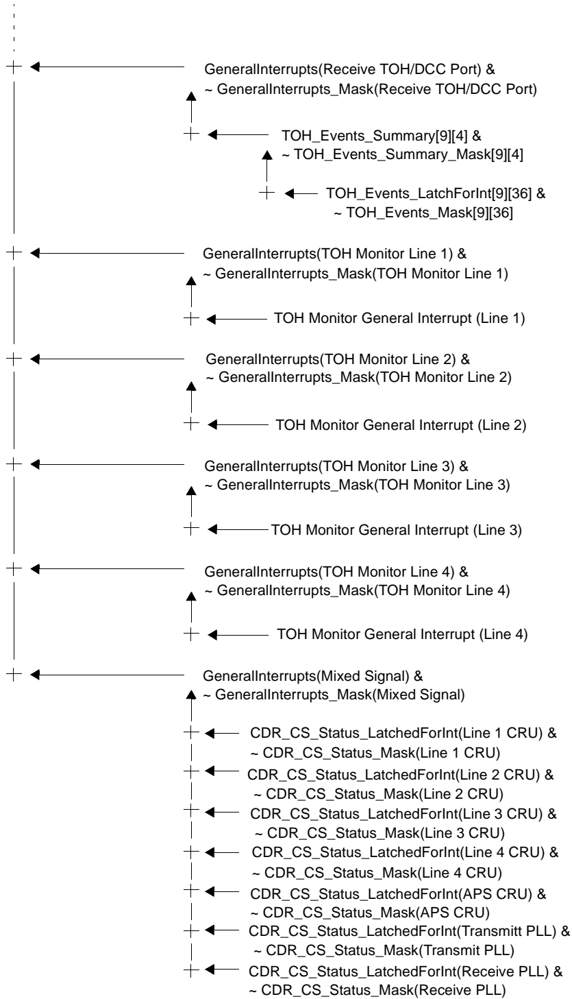
Figure 47. General Interrupt Tree (part 3)
