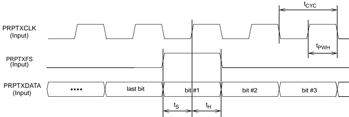
Figure 12. TX Path Alarm Indication Port Interface
