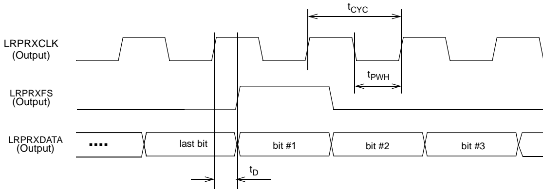
Figure 9. RX Line Ring Port Interface
