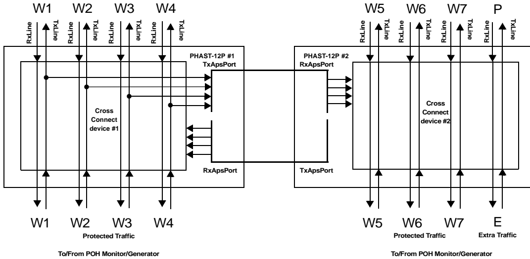
Figure 31. STM-1/OC-3, 1:7 APS Idle State
