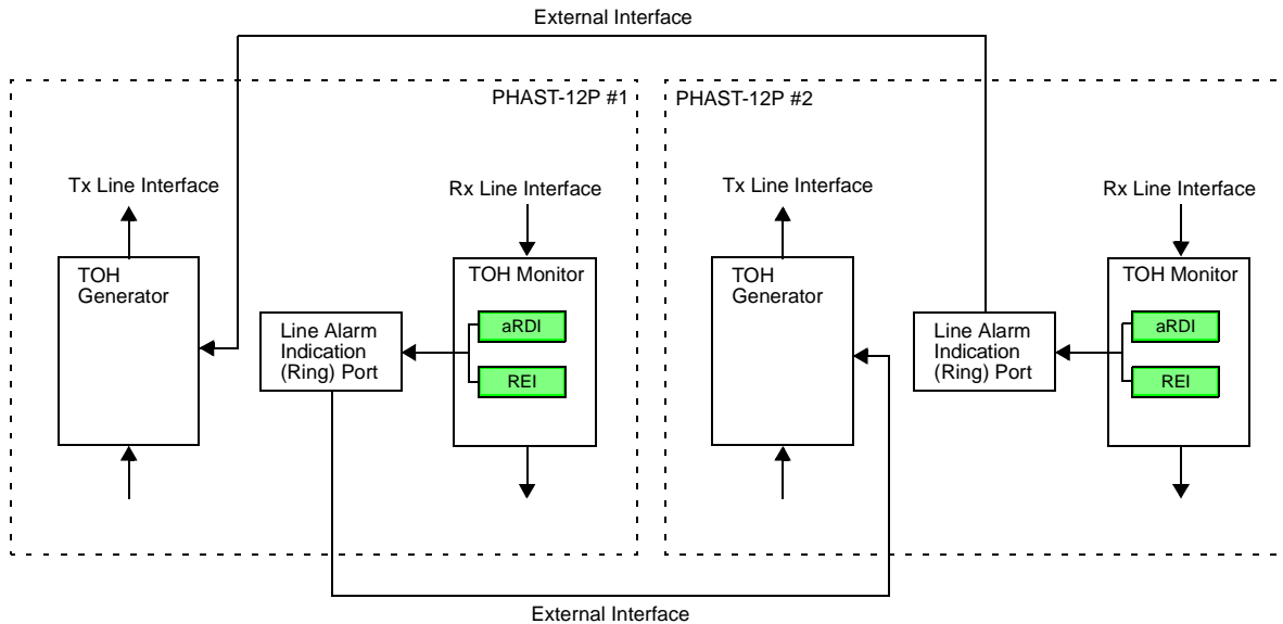
Figure 36. External Line Alarm Indication (Ring) Port Interface
