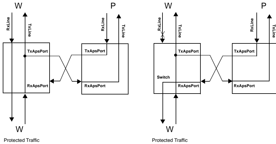
Figure 25. STM-4/OC-12, 1+1 APS
