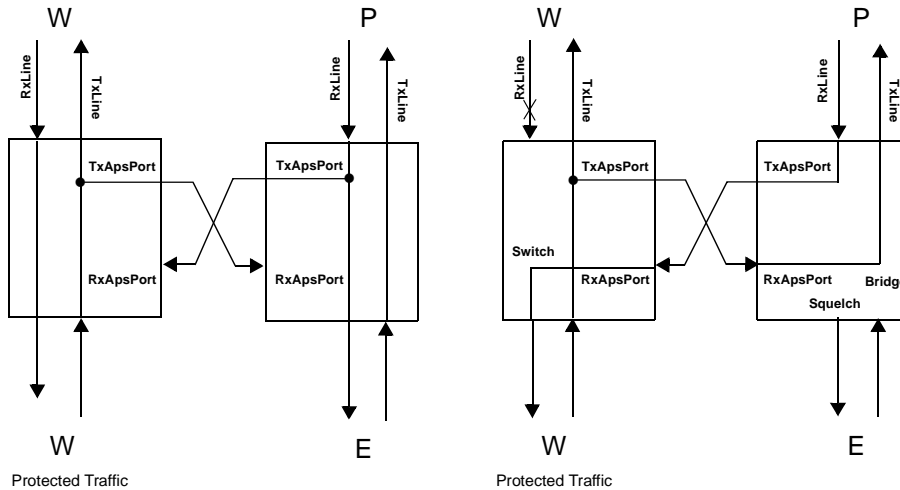
Figure 26. STM-4/OC-12, 1:1 APS
