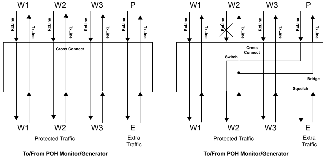
Figure 23. STM-1/OC-3, 1:3 APS with One PHAST-12P
