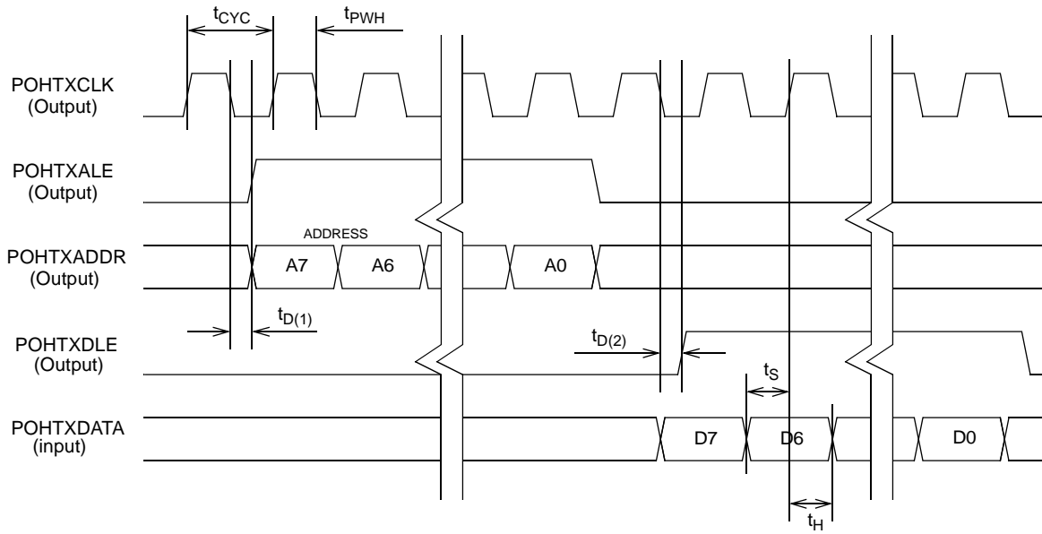
Figure 8. TX High Order POH Byte Interface
