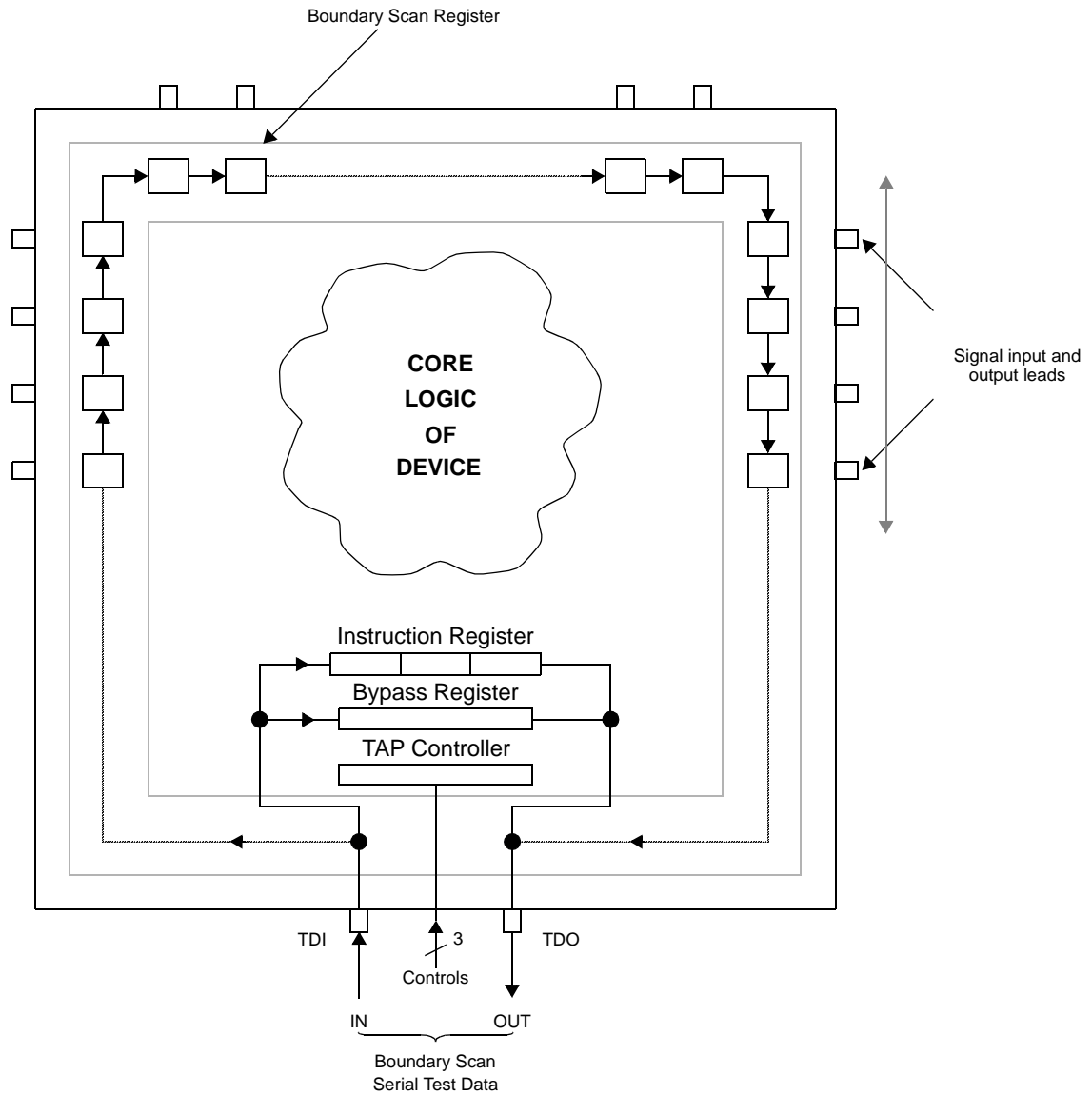
Figure 48. Boundary Scan Schematic
