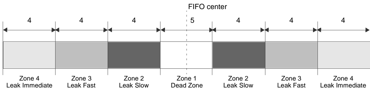
Figure 34. Retimer FIFO Filling Levels
