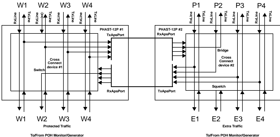
Figure 30. STM-1/OC-3, 1:1 APS Switch State
