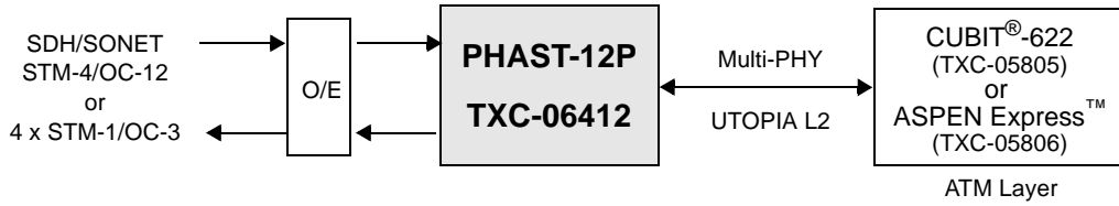
Figure 50. STM-4/OC-12 or 4 x STM-1/OC-3 ATM DSLAM Network Card
