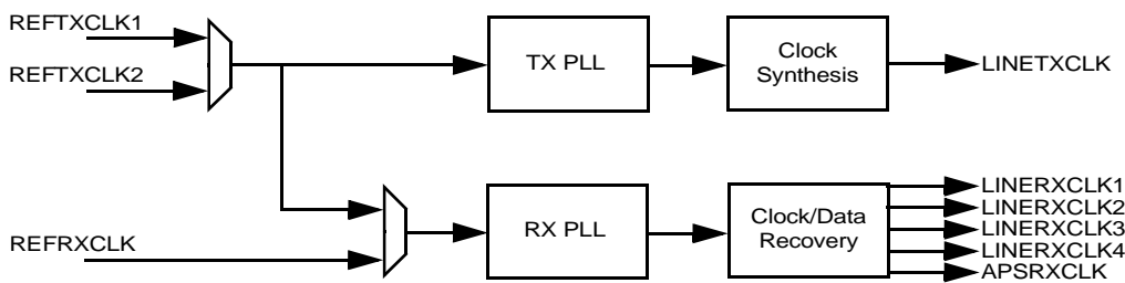
Figure 22. Clock Recovery and Clock Synthesis
