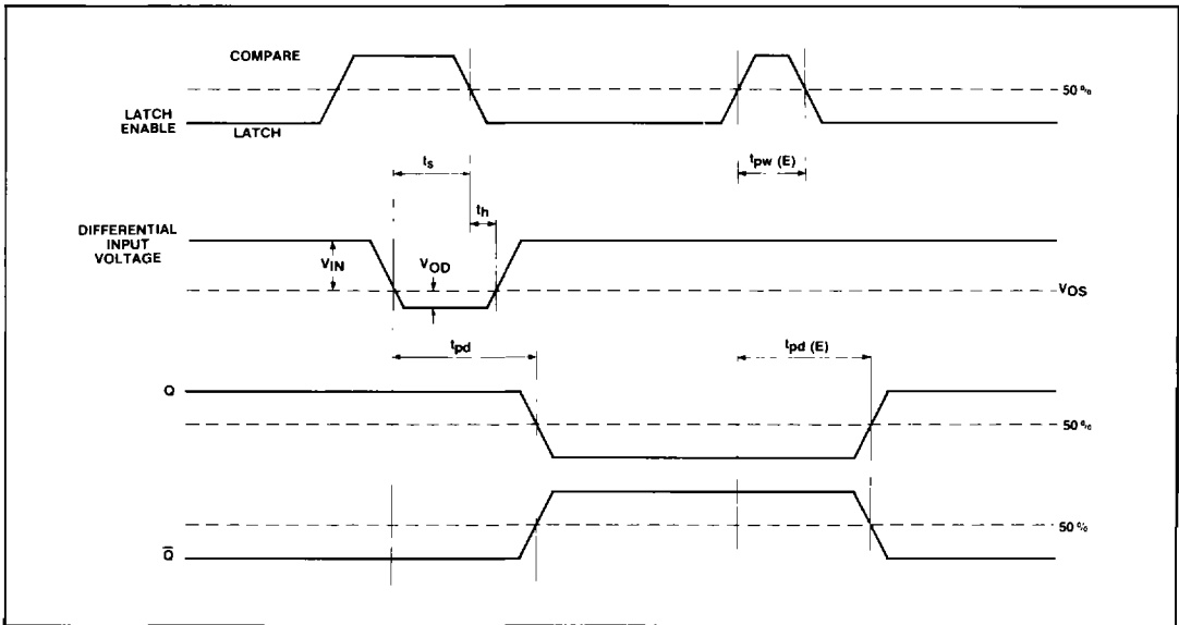
Fig.3 Timing diagram
