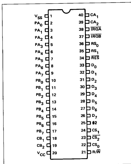
Figure 1. R6520 Pin Configuration
