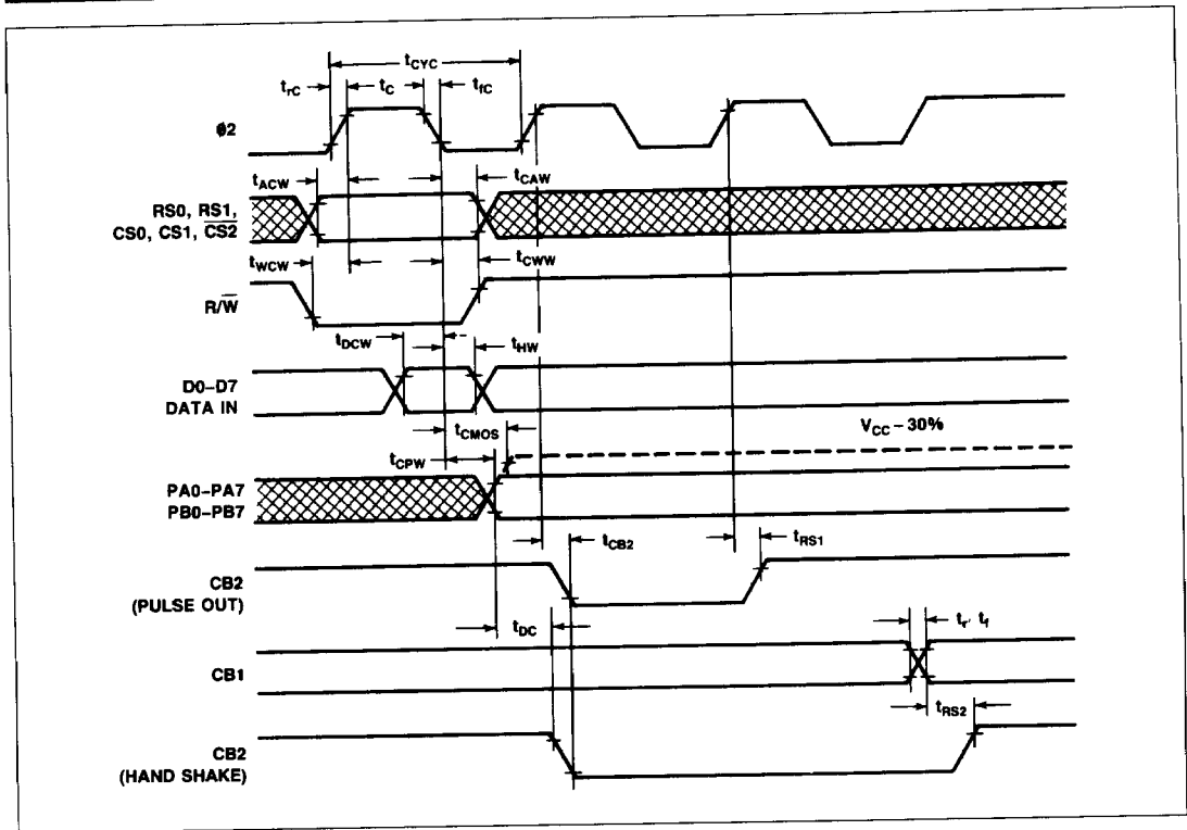
Figure 6. Write Timing Waveforms
