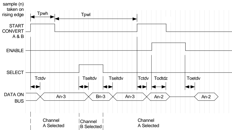
Figure 2. Timing Diagram
