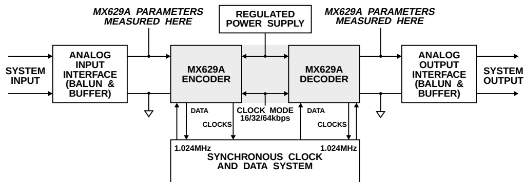
Figure 3: System Configuration using the MX629A
