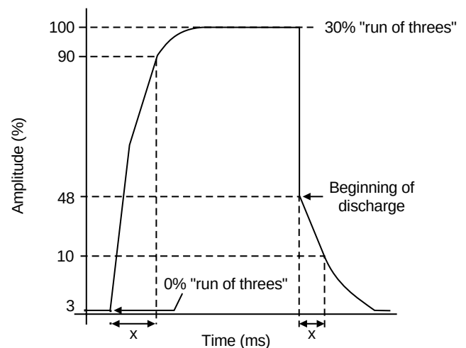
Figure 13: Compand Envelope
