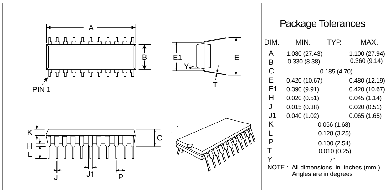
Figure 17: 22-pin PDIP (P) Mechanical Outline: Order as part no. MX629AP
