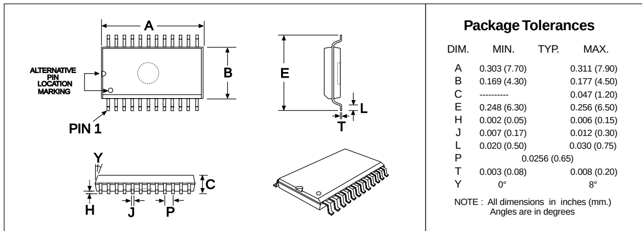
Figure 15: 24-pin TSSOP (TN) Mechanical Outline: Order as part no. MX629ATN
