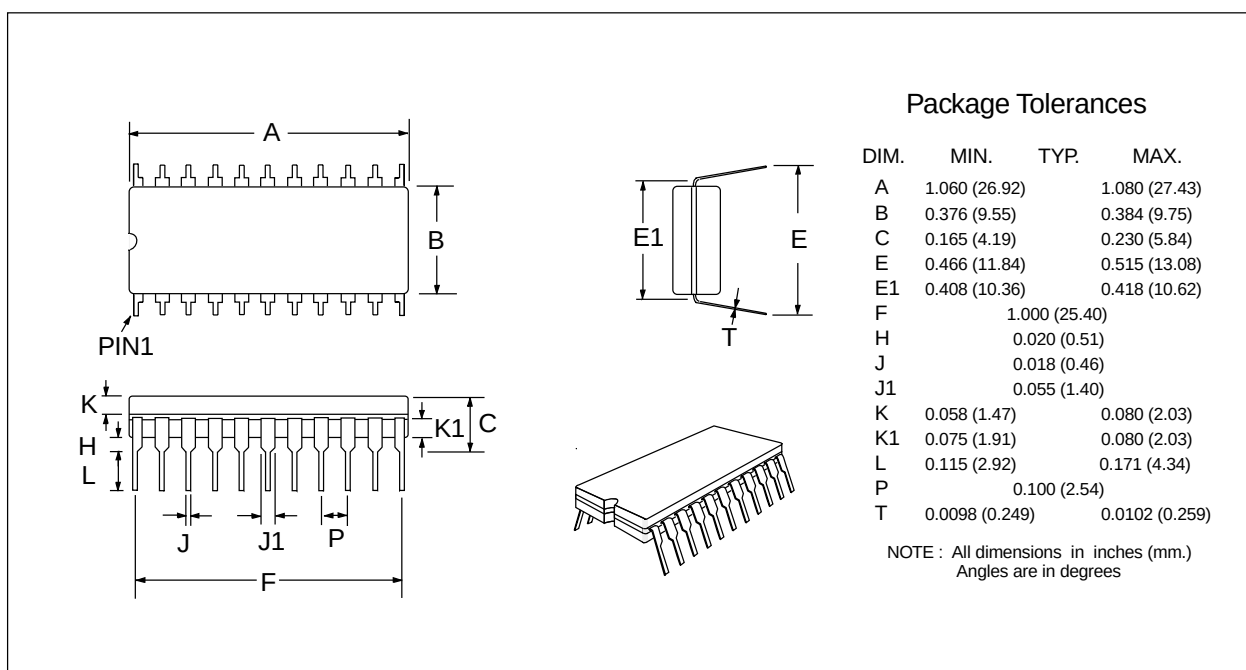
Figure 18: 22-pin Cerdip (J) Mechanical Outline: Order as part no. MX629AJ
