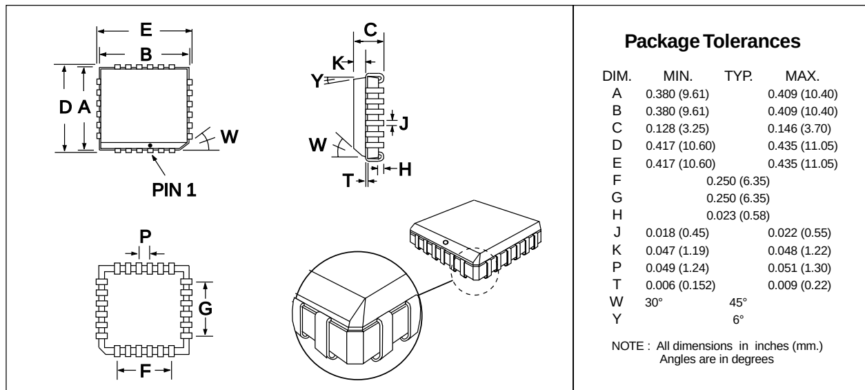
Figure 16: 24-pin PLCC (LH) Mechanical Outline: Order as part no. MX629ALH
