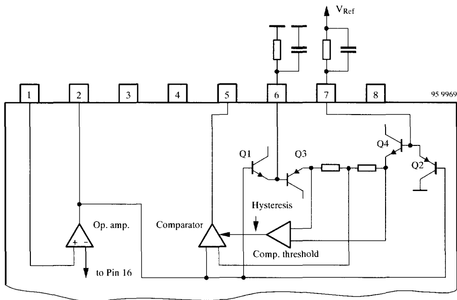
Figure 3. Principle function of the clamping comparator
