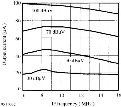
Figure 21. IF-frequency response
