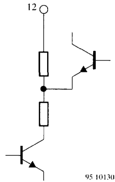
Figure 15. Pin 12 Discr
