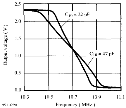
Figure 28. FM-discriminator characteristic
