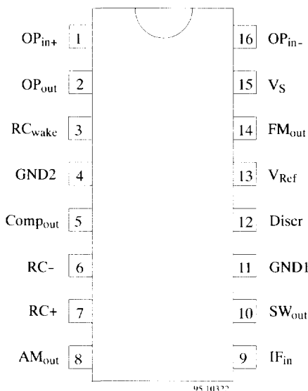
Figure 2. Pin description
