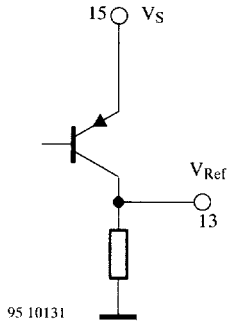
Figure 16. Pin 13 V_{Ref}
