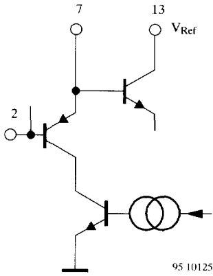
Figure 10. Pin 7 RC+
