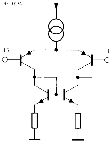
Figure 19. Pin 16 OP_{in-}
