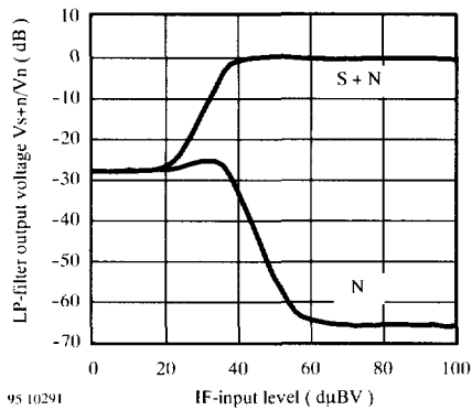
Figure 27. Signal-to-noise ratio FM: deviation 22.5 kHz
