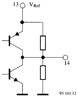
Figure 17. Pin 14 FM_{out}
