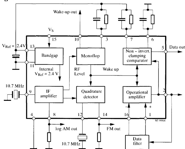
Figure 1. Block diagram
