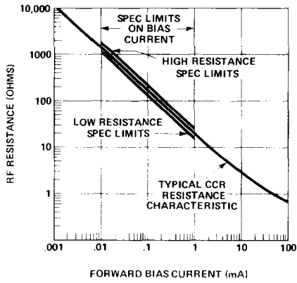
Figure 3. Typical RF Resistance vs. Bias for HPND-4165.
