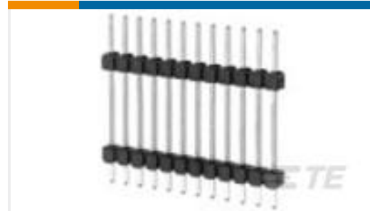
TE Model / Part #6-146459-4 14 MODII HDR SRST UNSHRD STKG
