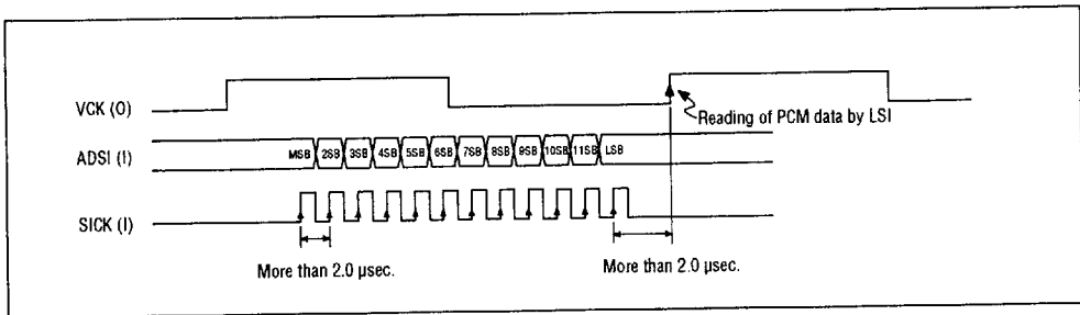
Figure 2-1 Use of External AD Converter and Timing
