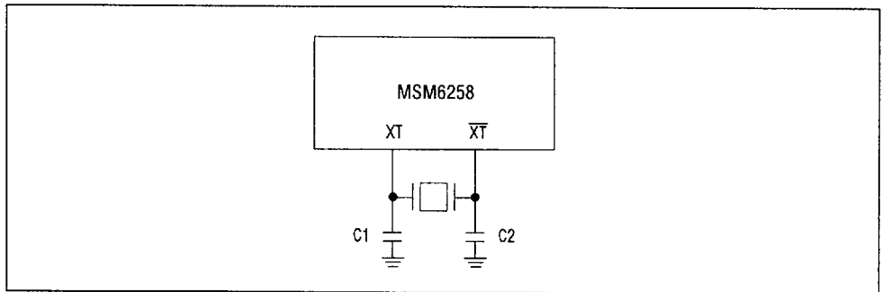
Figure 3 Connection of Oscillator
