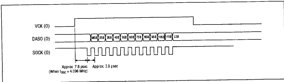
Figure 2-2 Use of External DA Converter and Timing
