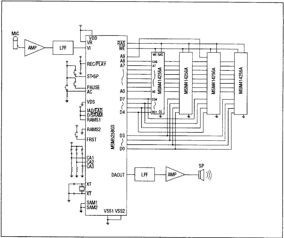
Figure 27 Application Note for 1M-bit DRAM
