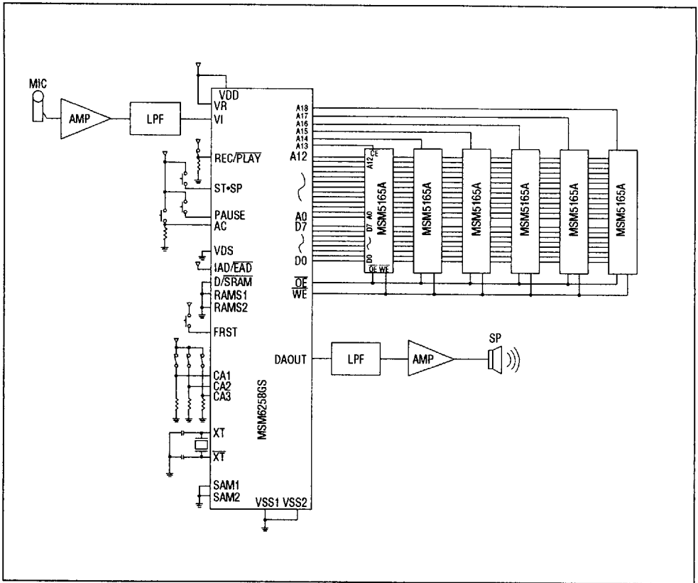
Figure 23 Application Note for 64K SRAM
