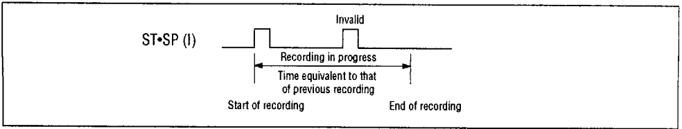
Figure 7 Recording in Status B (Preservation of Data in Channel)
