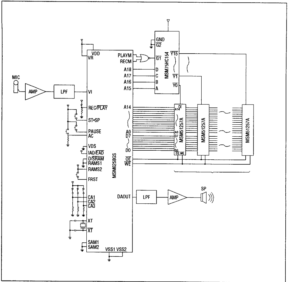
Figure 25 Application Note for 256K SRAM (Use 16 pcs)
