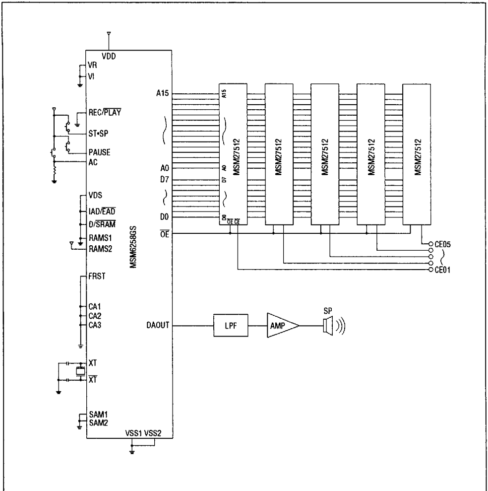
Figure 29 Application Note for 512K EPROM (Address is binary output)
