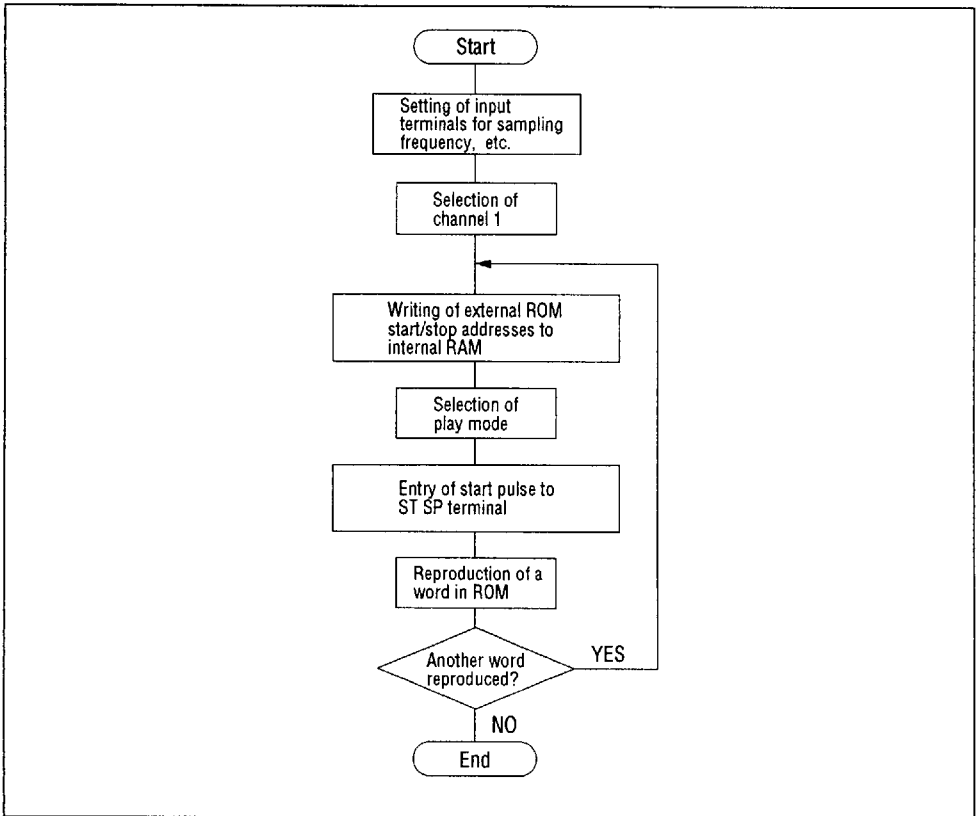
Figure 21 Flow Chart for Reproduction from ROM
