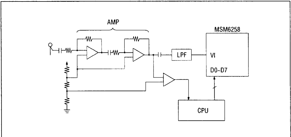
Figure 34 Voice-Triggered Starting Circuit for CPU Interface
