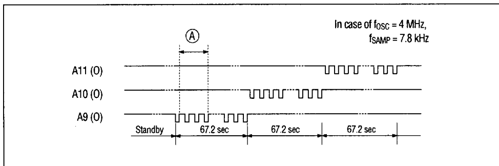
Figure 15 Address Timing for 256 x 4-Bit DRAM
