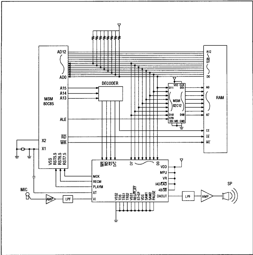
Figure 32 Example of Interface with MSM80C85
