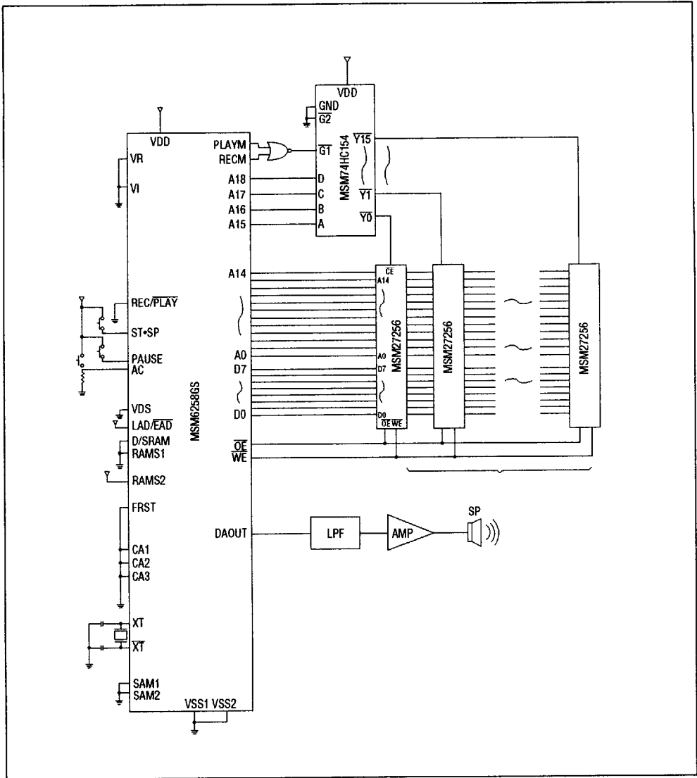
Figure 28 Application Note for 256K EPROM (Use 16 pcs)
