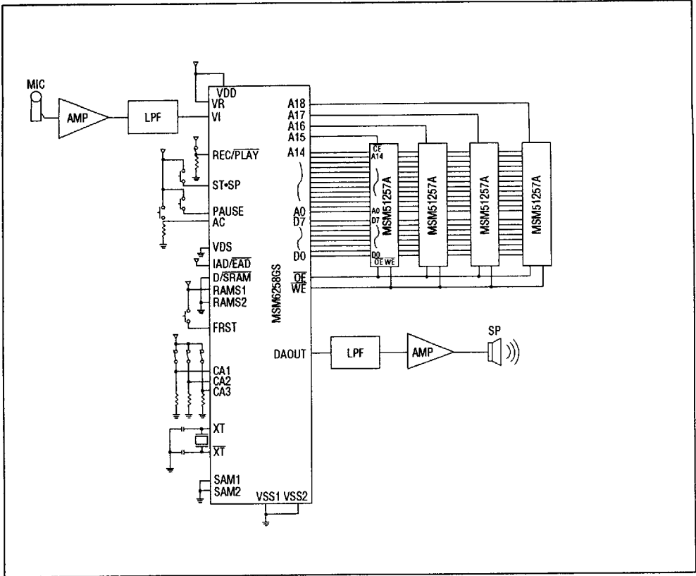
Figure 24 Application Note for 256K SRAM
