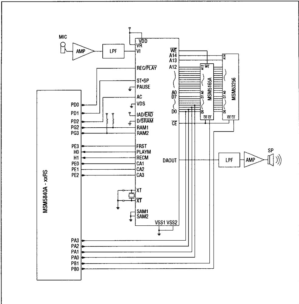
Figure 30 Example of Interface with 64K SRAM & 256K Mask ROM
