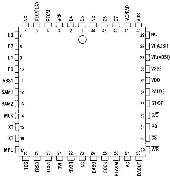
(Top View) 44-Pin Plastic Leaded Chip Carrier
