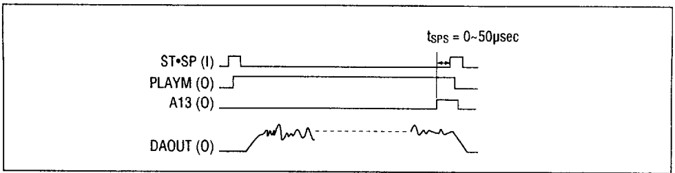
Figure 20 Stop Timing for Reproduction from ROM
