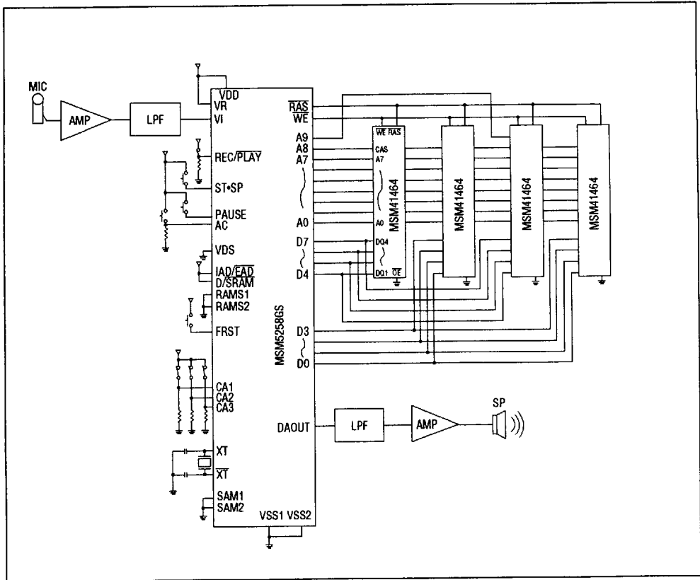
Figure 26 Application Note for 256K DRAM
