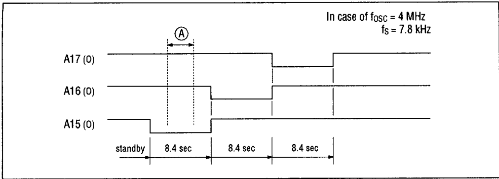
Figure 18 Address Timing for 256K SRAM
