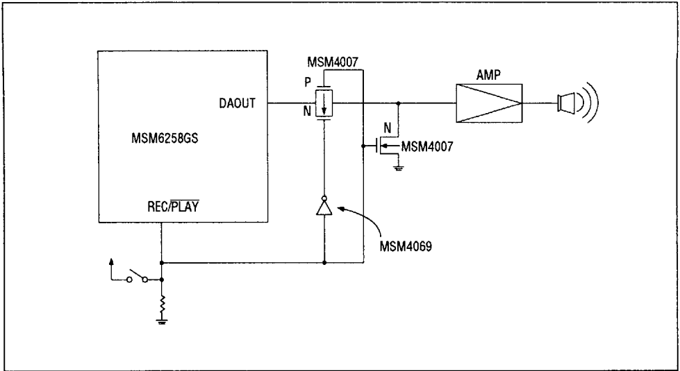
Figure 33 Example of Mute Circuit for Recording
