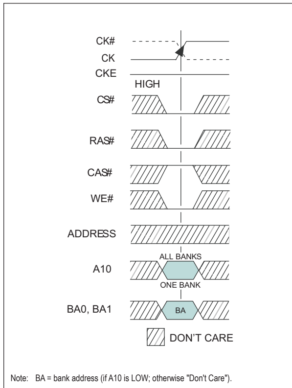
FIGURE 13 – PRECHARGE COMMAND
