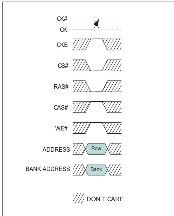
FIGURE 10 – ACTIVE COMMAND
