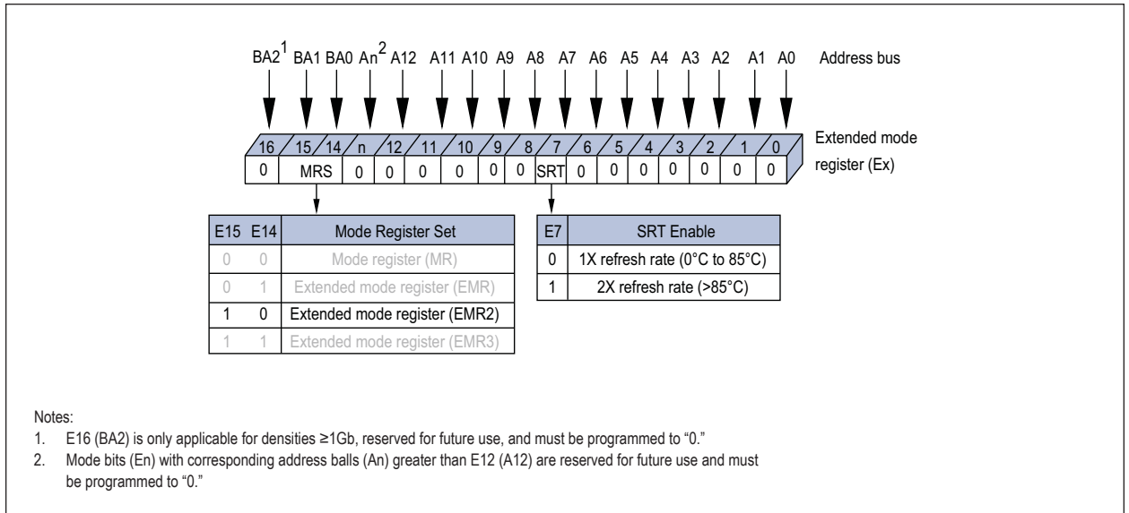
FIGURE 8 – EXTENDED MODE REGISTER 2 (EMR2) DEFINITION
