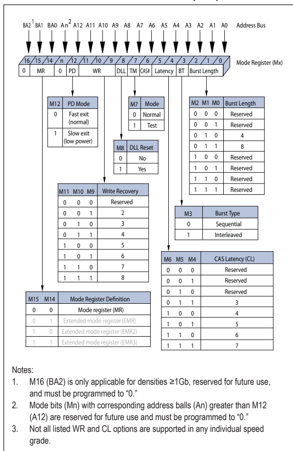
FIGURE 5 – MODE REGISTER (MR) DEFINITION
