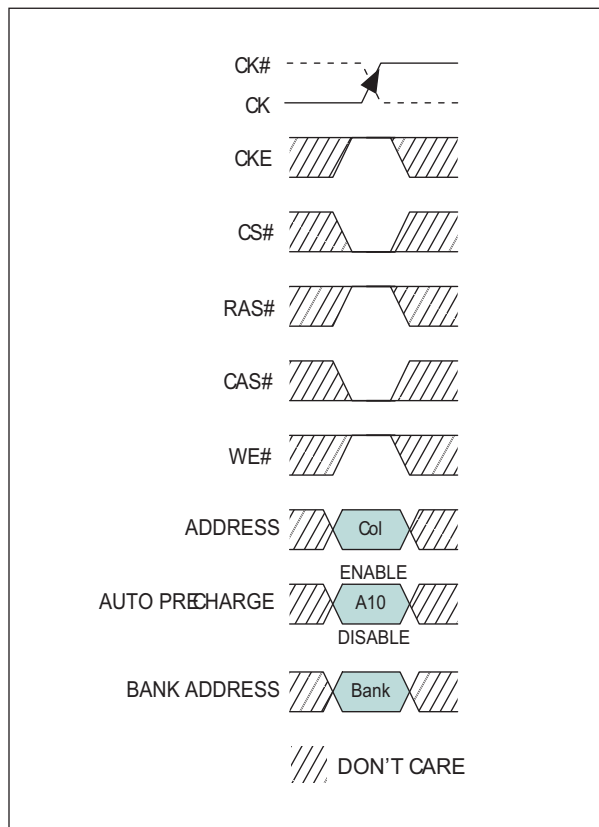
FIGURE 11 – READ COMMAND
