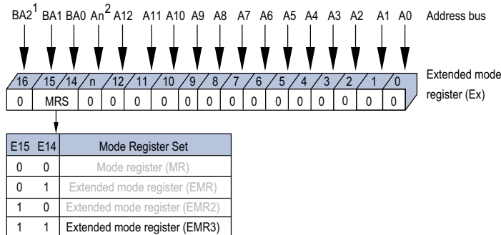
FIGURE 9 – EXTENDED MODE REGISTER 3 (EMR3) DEFINITION
