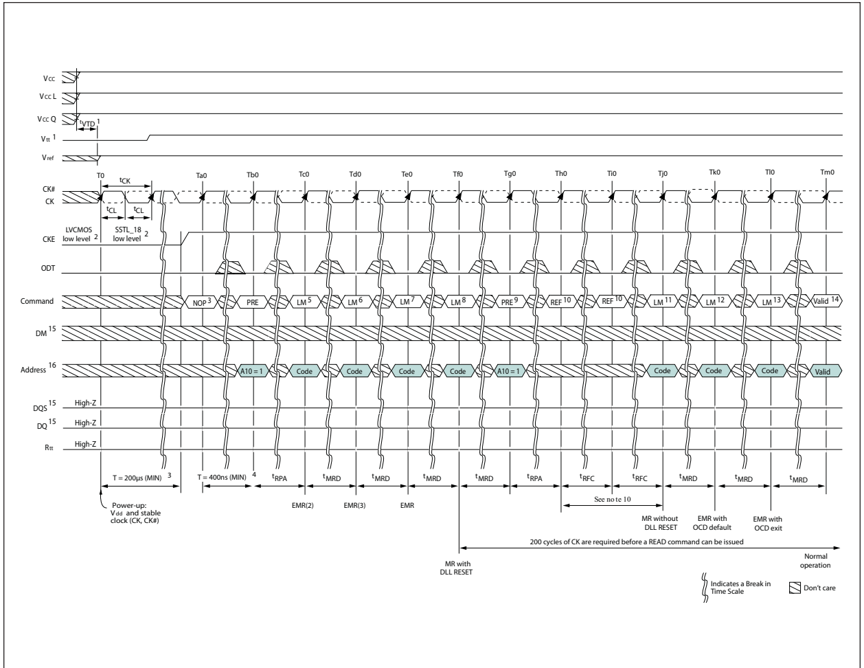
FIGURE 4 – POWER-UP AND INITIALIZATION
