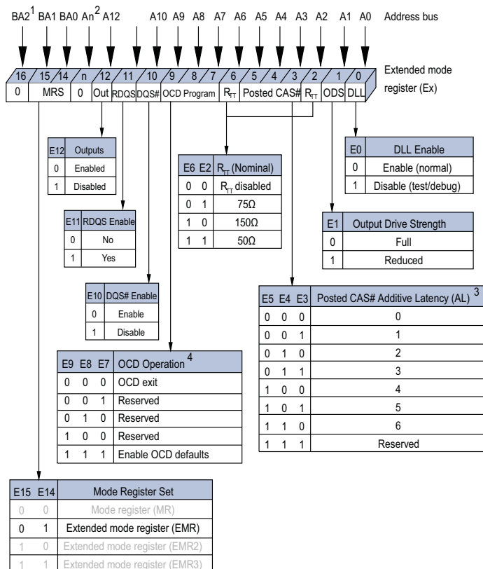
FIGURE 7 – EXTENDED MODE REGISTER DEFINITION
