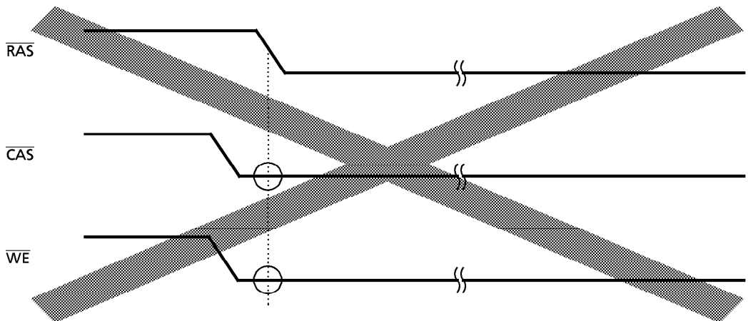
WCBR timing
