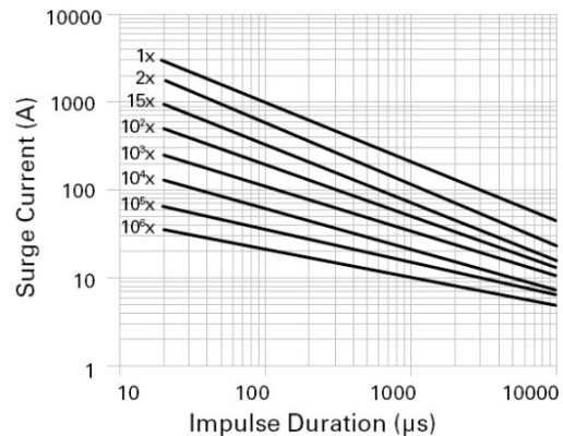
Repetitive Surge Capability for 14mm Parts V14x11P - V14x40P
