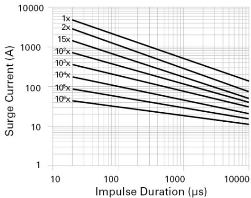
Repetitive Surge Capability for 20mm Parts V20x11P - V20x40P
