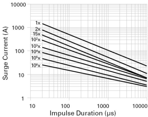
Repetitive Surge Capability for 10mm Parts V10x11P - V10x40P
