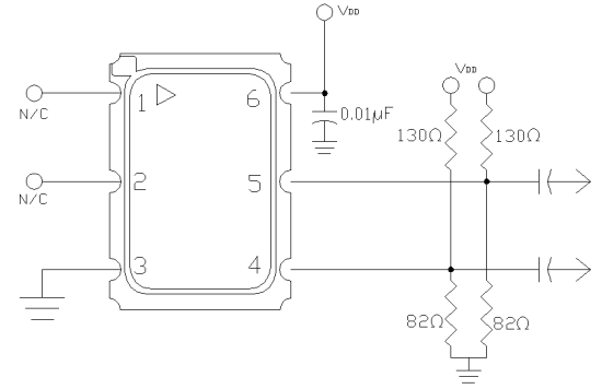
Figure 9. Pull-Up Pull Down Termination Resistor values are typically for 3.3V operation For 2.5V operation, the resistor to ground is 62 ohms and the resistor to supply is 240 ohms
