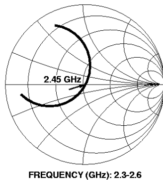
Figure 20. Input Impedance, Modified 2.45 GHz Circuit.
