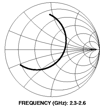
Figure 18. Input Impedance.
