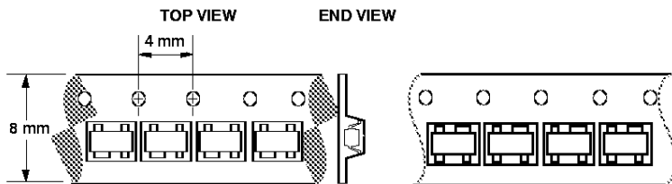
Figure 29. Options T31, L31 for SOT-143 Packages.
