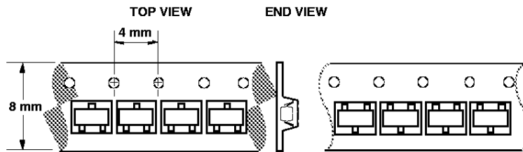
Figure 27. Options T31, L31, for SOT-23 Packages.
