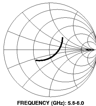
Figure 23. Input Impedance.
