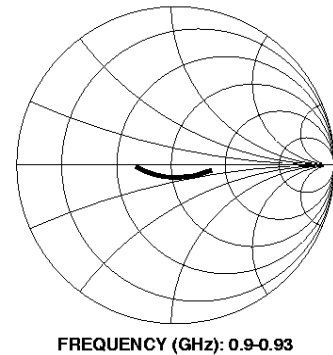
Figure 12. Input Impedance.
