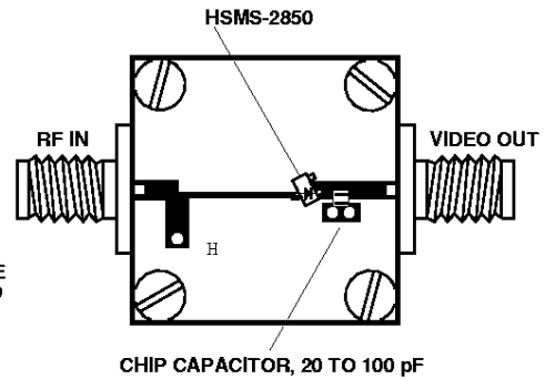
Figure 17. Test Detector.
