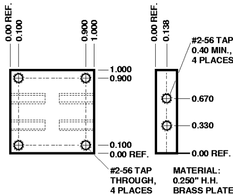
Figure 16. Mounting Plate.
