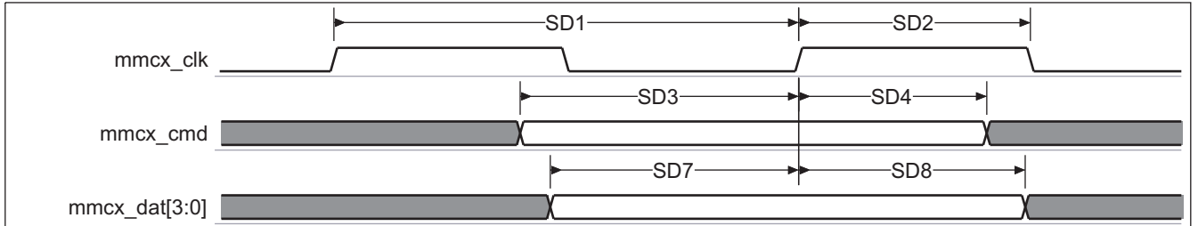
Figure 6-61. MMC/SD/SDIO – Standard SD Mode – Data/Command Receive
