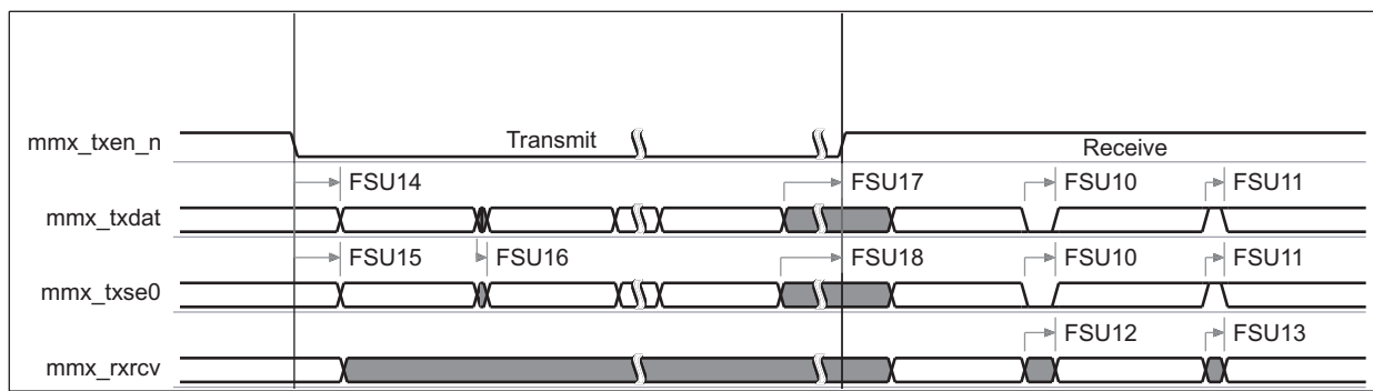
Figure 6-38. Low-/Full-Speed USB – Bidirectional Standard 4-pin Mode
