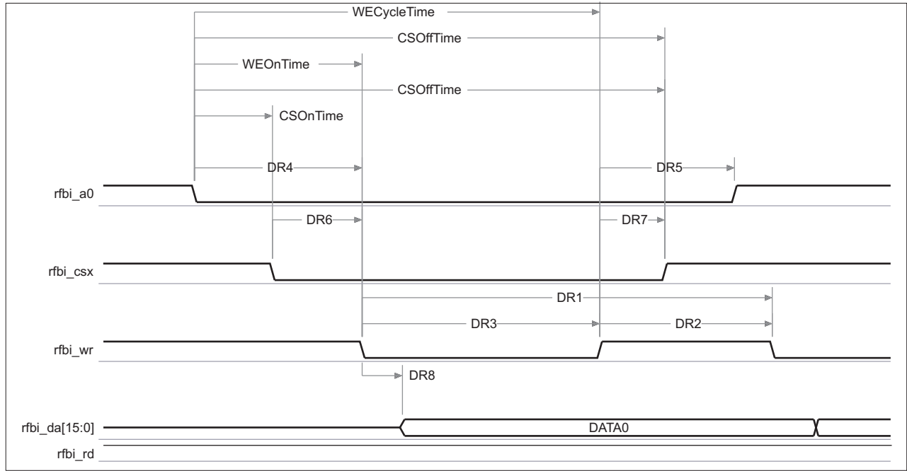
Figure 6-26. LCD Display Interface in RFBI Mode – Data Read-to-Write and Write-to-Read Modes (1)(2)
