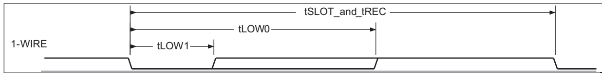
Figure 6-55. 1-Wire Write Bit Timing (Command/Address or Data)
