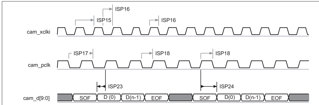
Figure 6-21. ISP – ITU Mode (1)(2)
