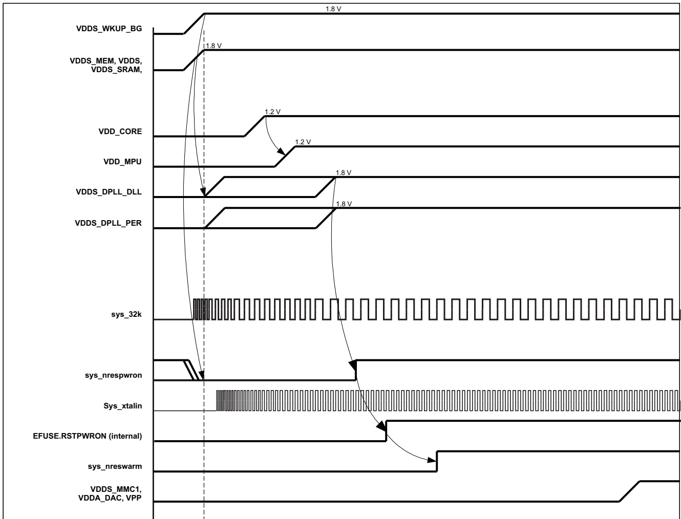
Figure 3-3. Power-up Sequence
