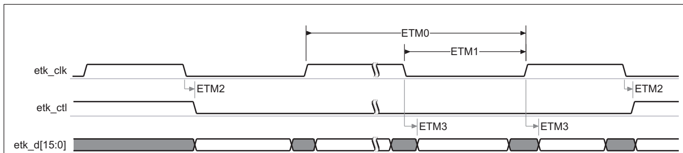
Figure 6-63. Embedded Trace Macro Interface
