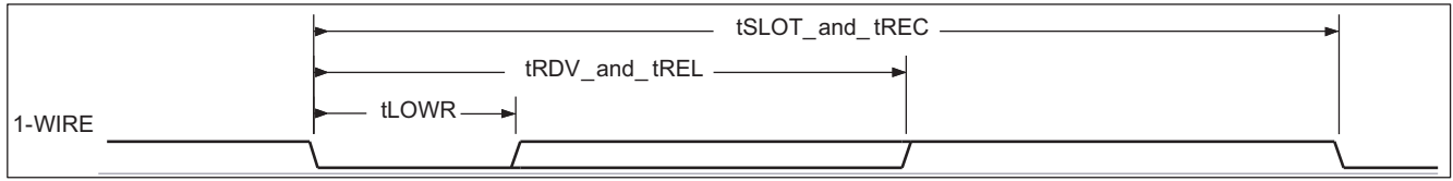
Figure 6-54. 1-Wire Read Bit Timing (Data)
