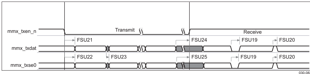
Figure 6-39. Low-/Full-Speed USB – Bidirectional Standard 3-pin Mode
