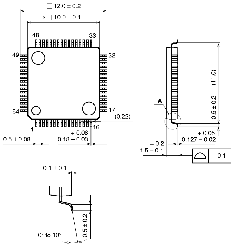
DETAIL A
