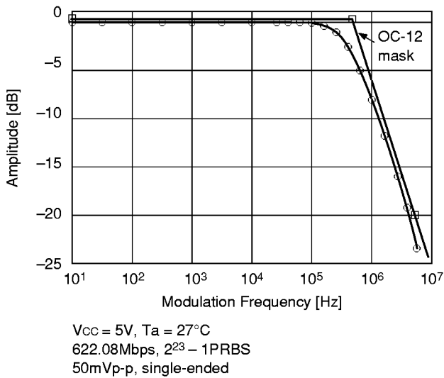
Fig. 12. Jitter transfer function
