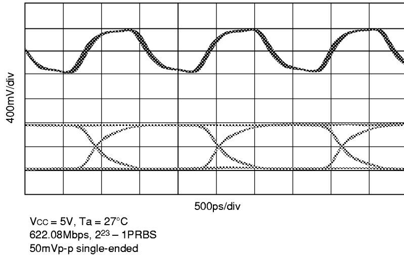
Fig. 10. RCK/RDATA output waveform
