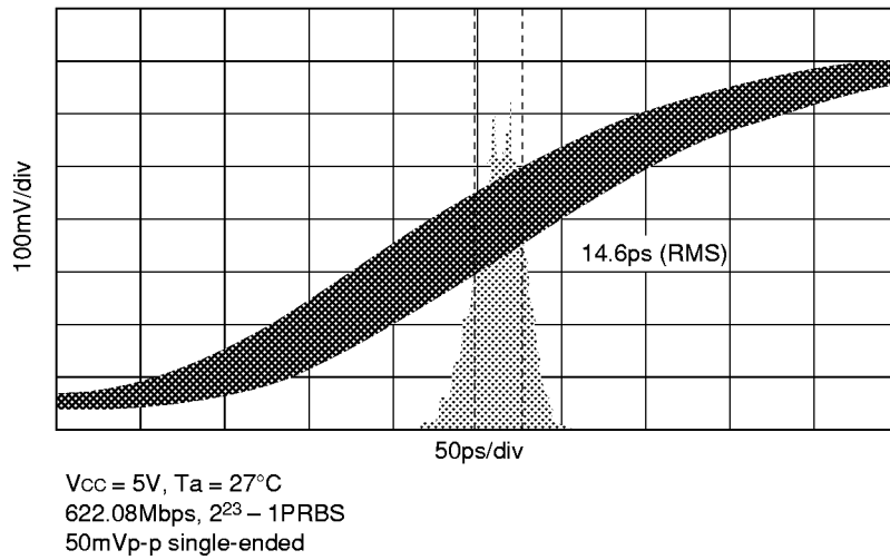
Fig. 11. RCK output histogram
