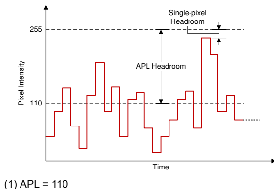
Figure 7-10. Source Pixels for a Color Channel
