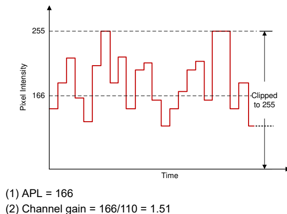
Figure 7-11. Pixels for a Color Channel After CAIC Processing
