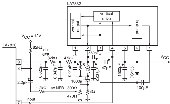
LA7820 vertical output
