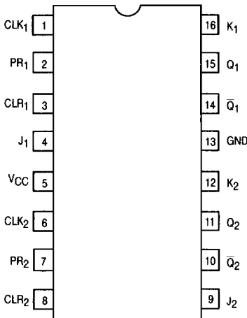
CONNECTION DIAGRAM
