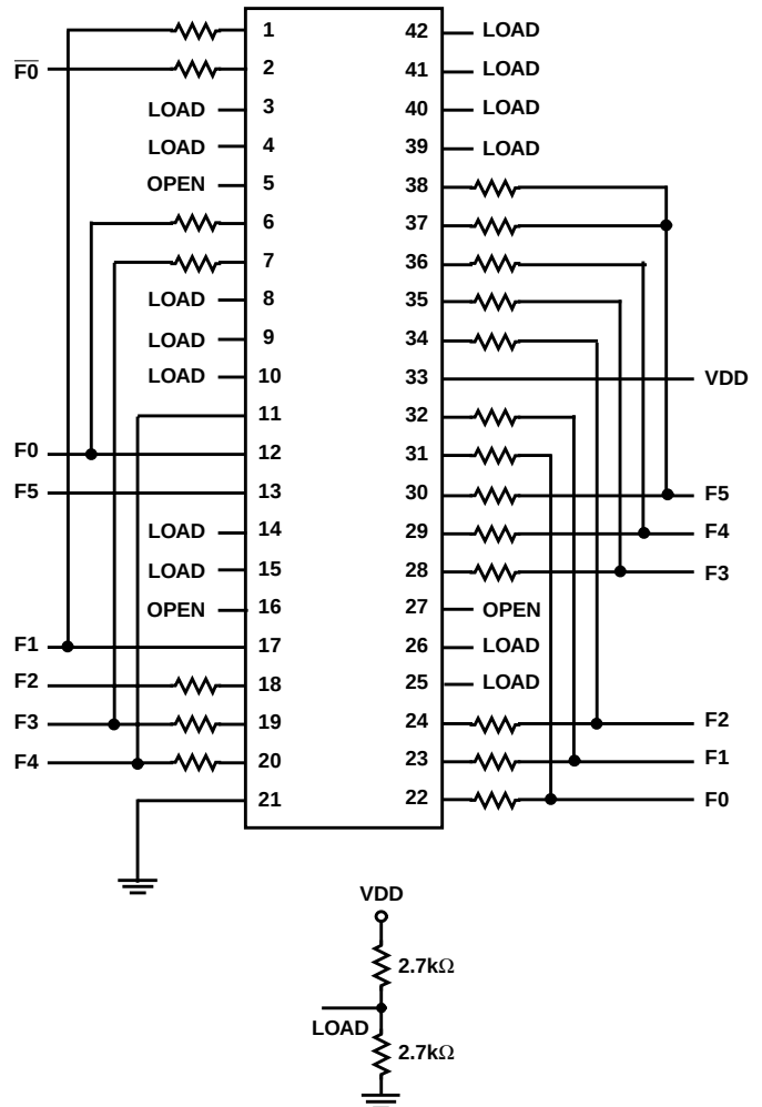
HS-82C37ARH 42 LEAD CERAMIC FLATPACK
