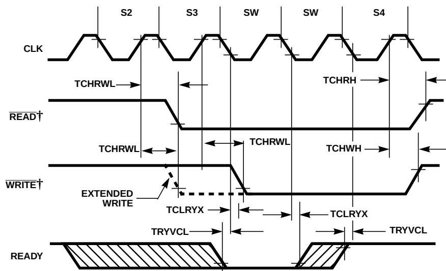
FIGURE 3. READY
