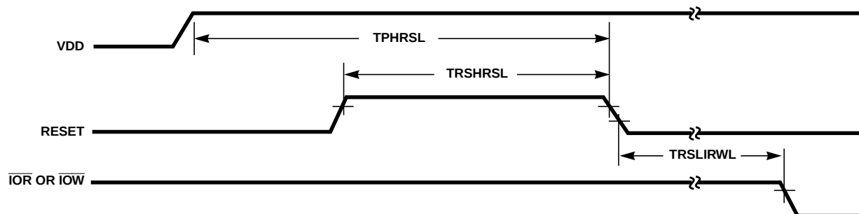
FIGURE 6. RESET
