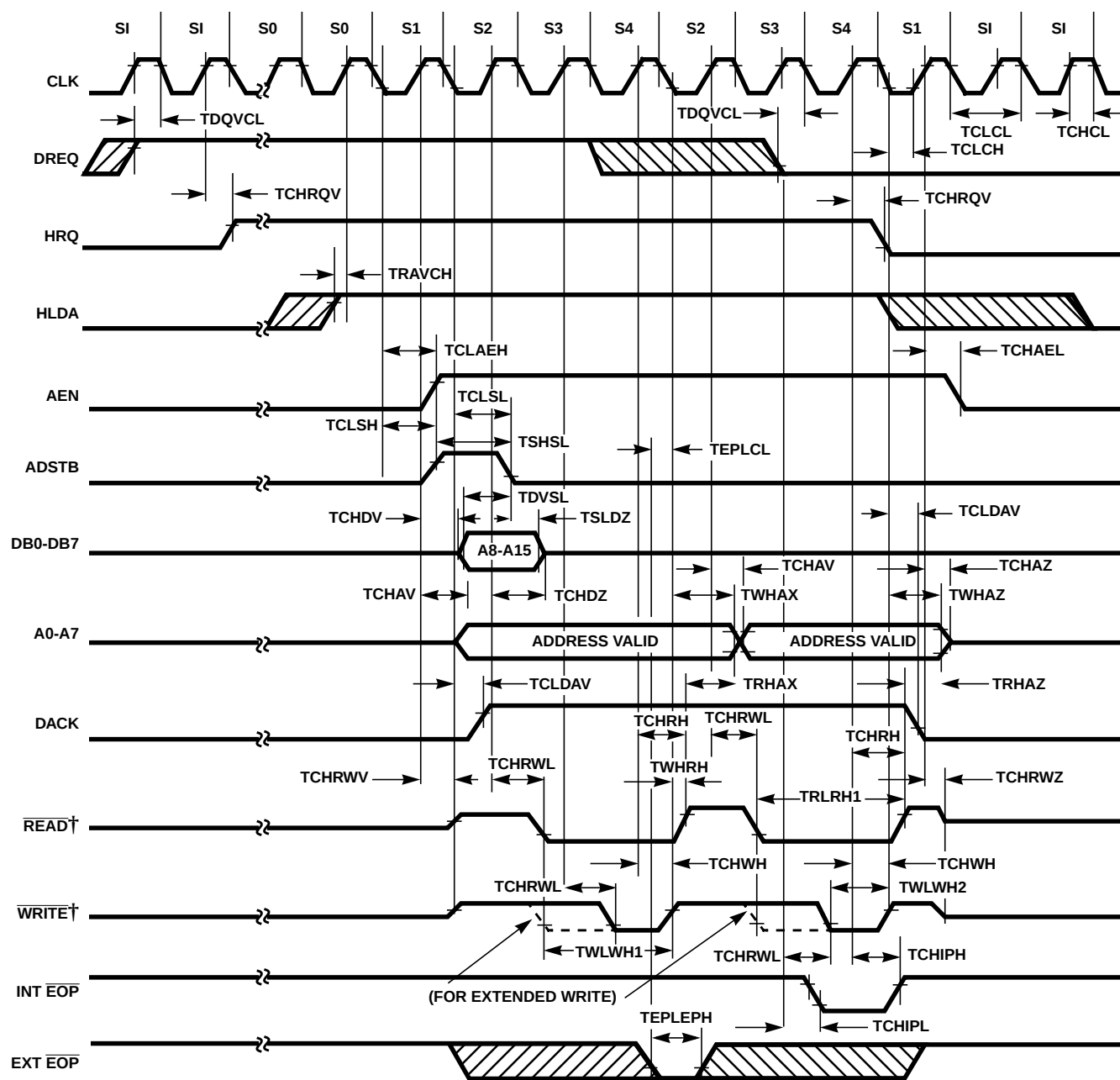
FIGURE 4. DMA TRANSFER
