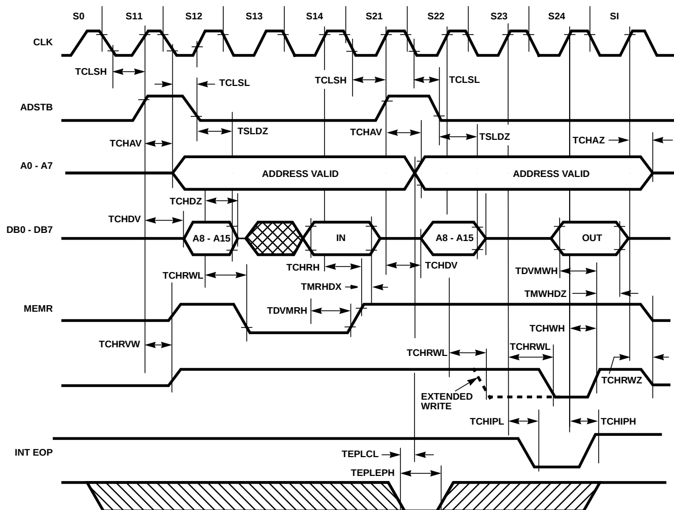
FIGURE 5. MEMORY-TO-MEMORY TRANSFER
