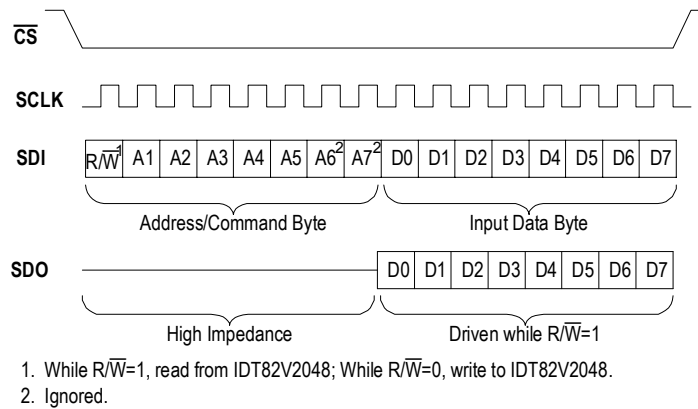
Figure-20 Serial Host Mode Timing
