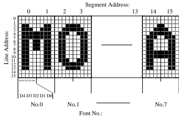
Figure 11. Memory Map of Programmable RAM Fonts
