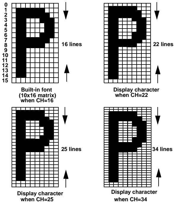
Figure 12. Variable Character Height
