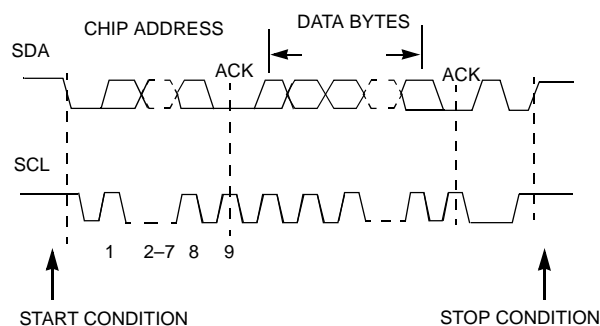
Figure 2. M_BUS Format
