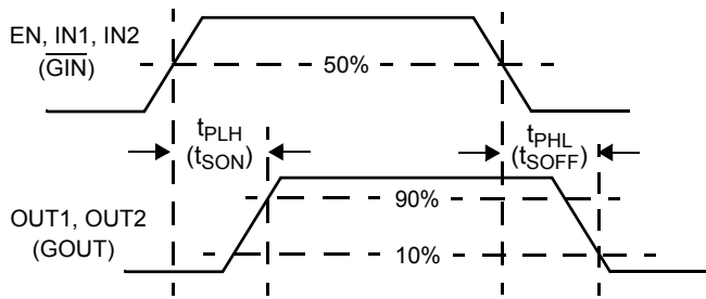
Figure 2. t_{PLH} , t_{PHL} , and t_{PZH} Timing
