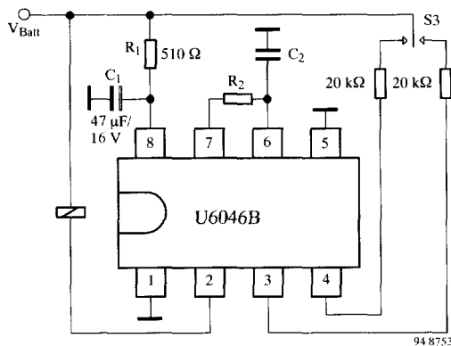
Figure 7. ON/OFF function U6046B
