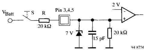
Figure 10. Input circuit U6046B
