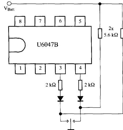
Figure 15. Increasing the contact current by parallel resistors
