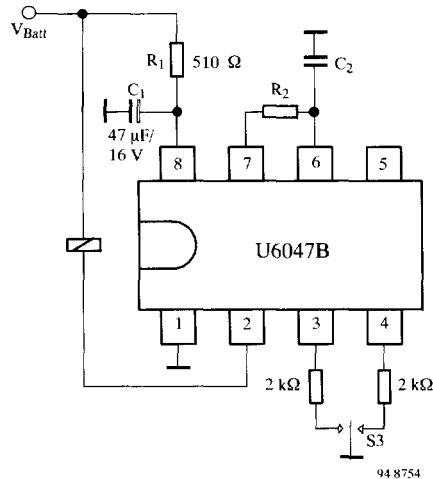
Figure 8. ON/OFF function U6047B
