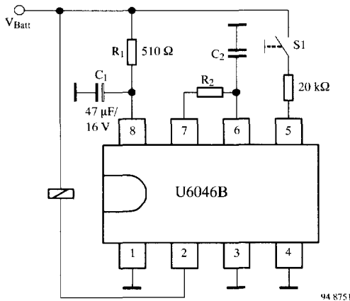
Figure 5. TOGGLE function U6046B
