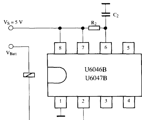
Figure 4. Basic circuit for V_S = 5 \text{ V}
