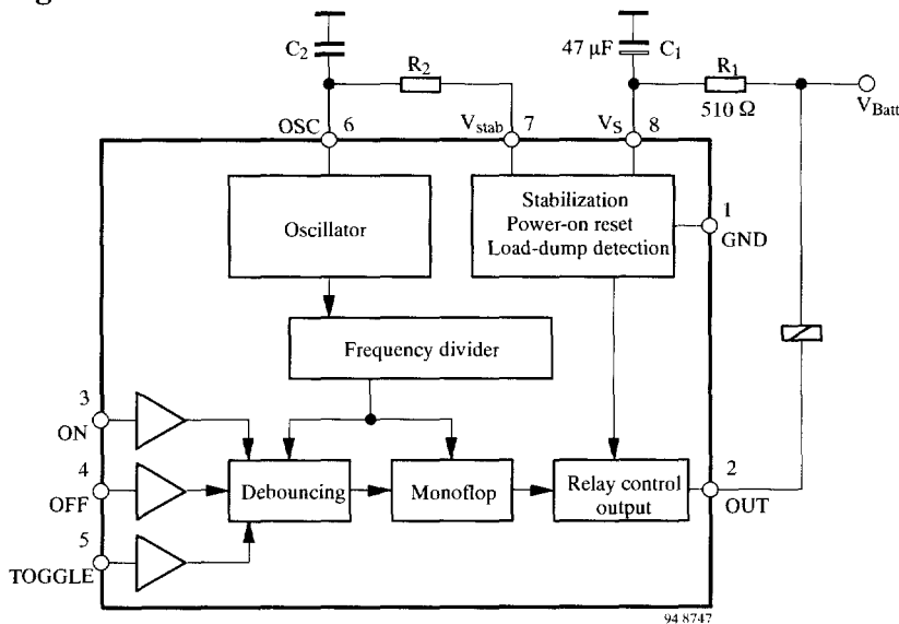
Figure 1. Block diagram with external circuit
