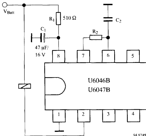
Figure 3. Basic circuit for 12 V supply and oscillator
