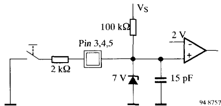
Figure 11. Input circuit U6047B
