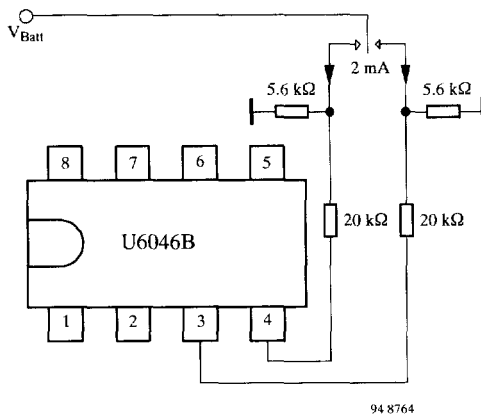
Figure 15. Increasing the contact current by parallel resistors
