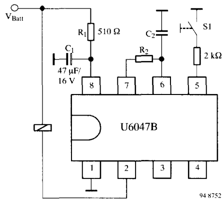
Figure 6. TOGGLE function U6047B
