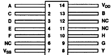
14-Lead Flatpack Top View
