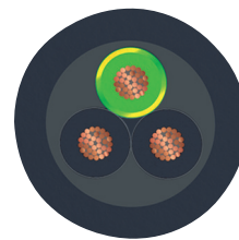
PUR/PVC, 0.75 mm 2 , black [116]
