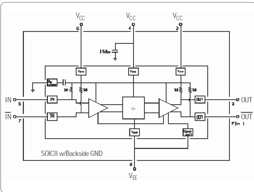
Figure 1. Simplified Schematic
