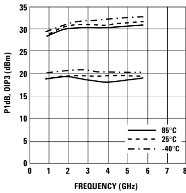
Figure 15. P1dB, OIP3 vs. Frequency and Temp at Vd = 4V, Ids = 60 mA.
