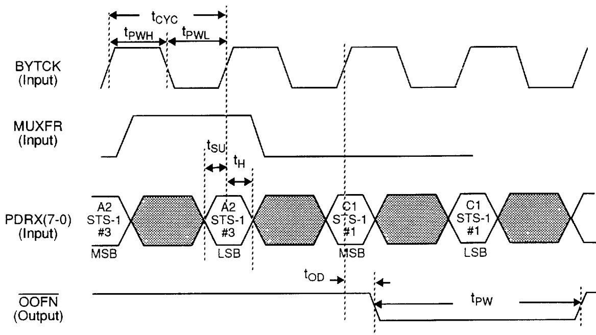
Figure 7. STS-3 Nibble Receive Timing
