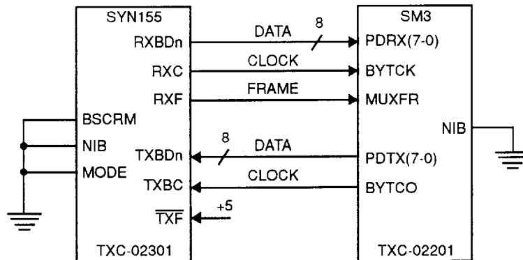
Figure 11. SM3/SYN155 Interface
