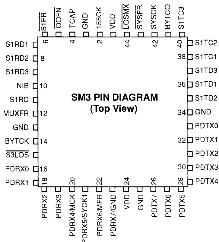
Figure 3. SM3 Pin Diagram with Numbers and Names
