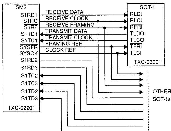
Figure 10. SM3/SOT-1 Interface
