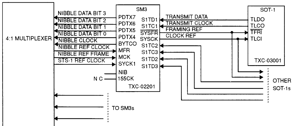
Figure 13. OC-12 Reference Timing Interface
