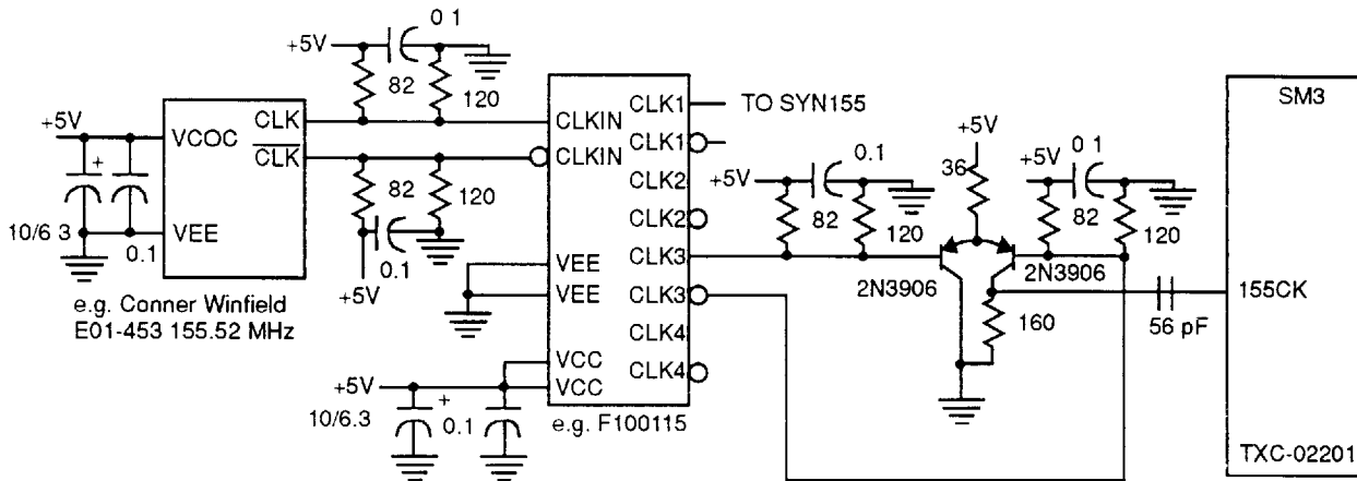
Figure 12. SM3 Clock Interface
