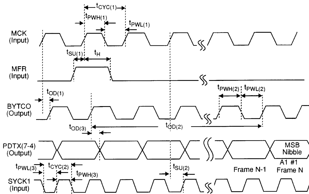
Figure 5. STS-3 Nibble Transmit Timing
