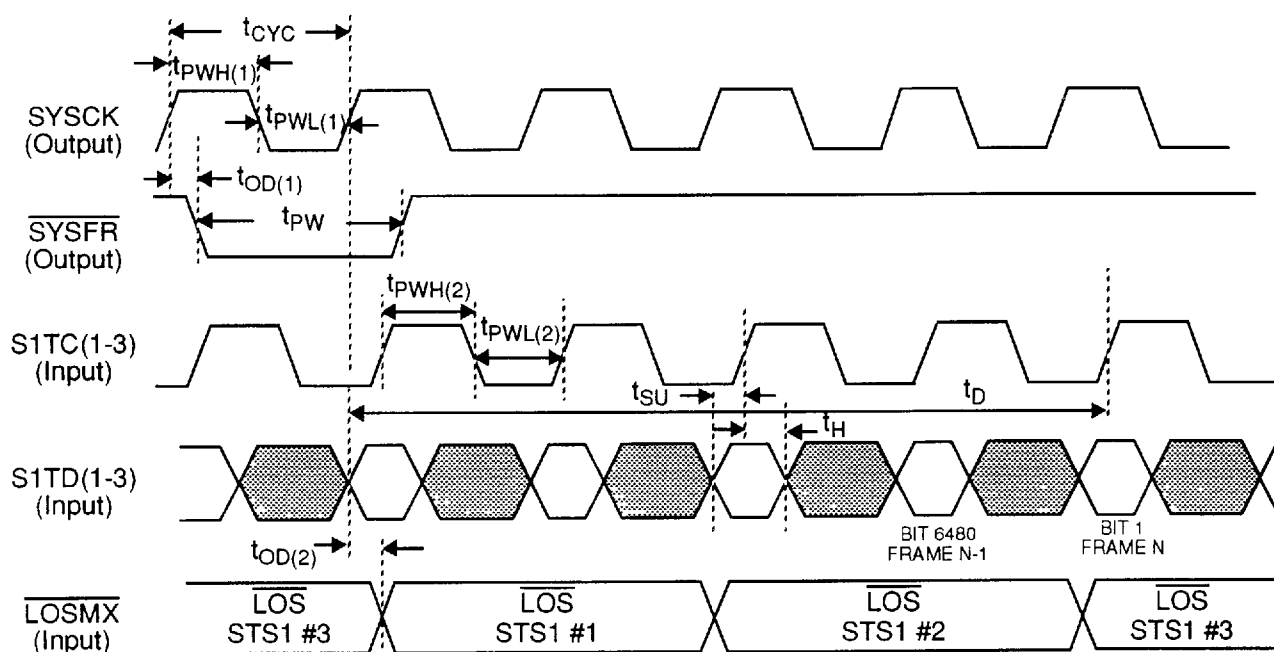
Figure 9. STS-1 Transmit Timing
