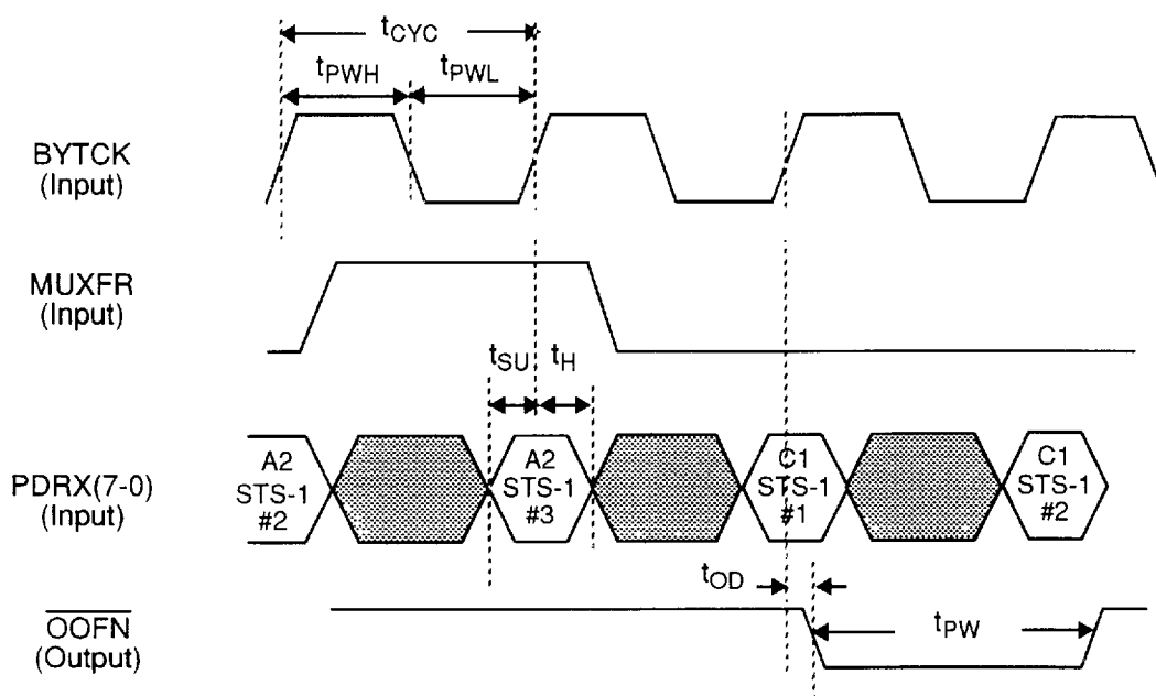
Figure 6. STS-3 Byte Receive Timing
