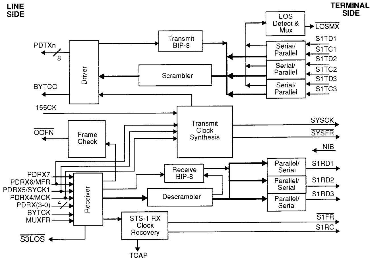
Figure 1. SM3 Block Diagram
