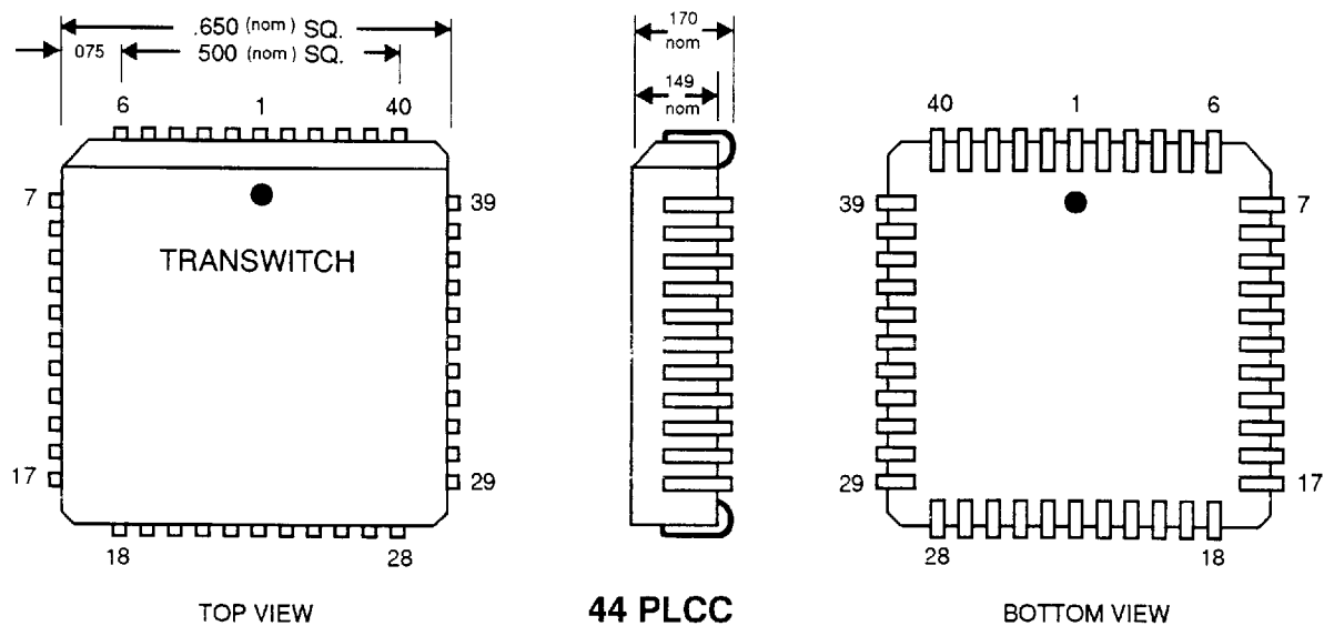
Figure 14. SM3 44-Pin Plastic Leaded Chip Carrier
