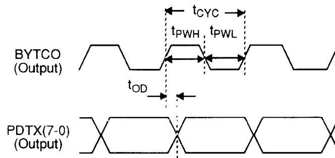
Figure 4. STS-3 Byte Transmit Timing
