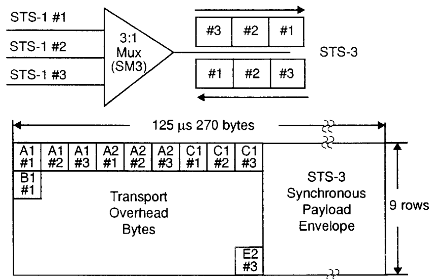
Figure 2. STS-3 Format
