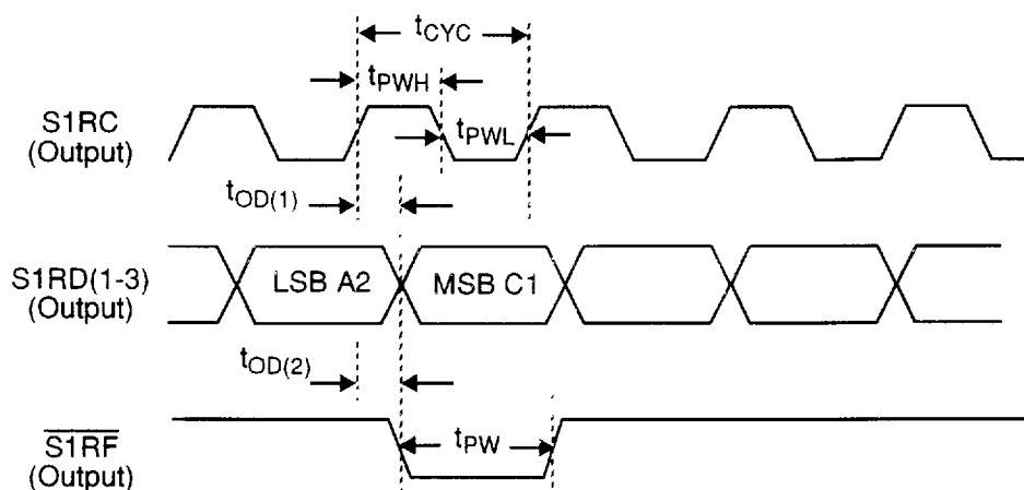
Figure 8. STS-1 Receive Timing
