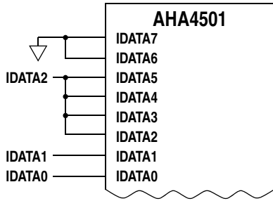
Figure 2: IDATA Interface
