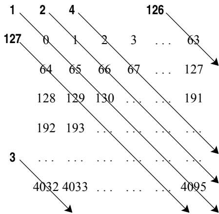
Figure 4: 2D Interleaving
