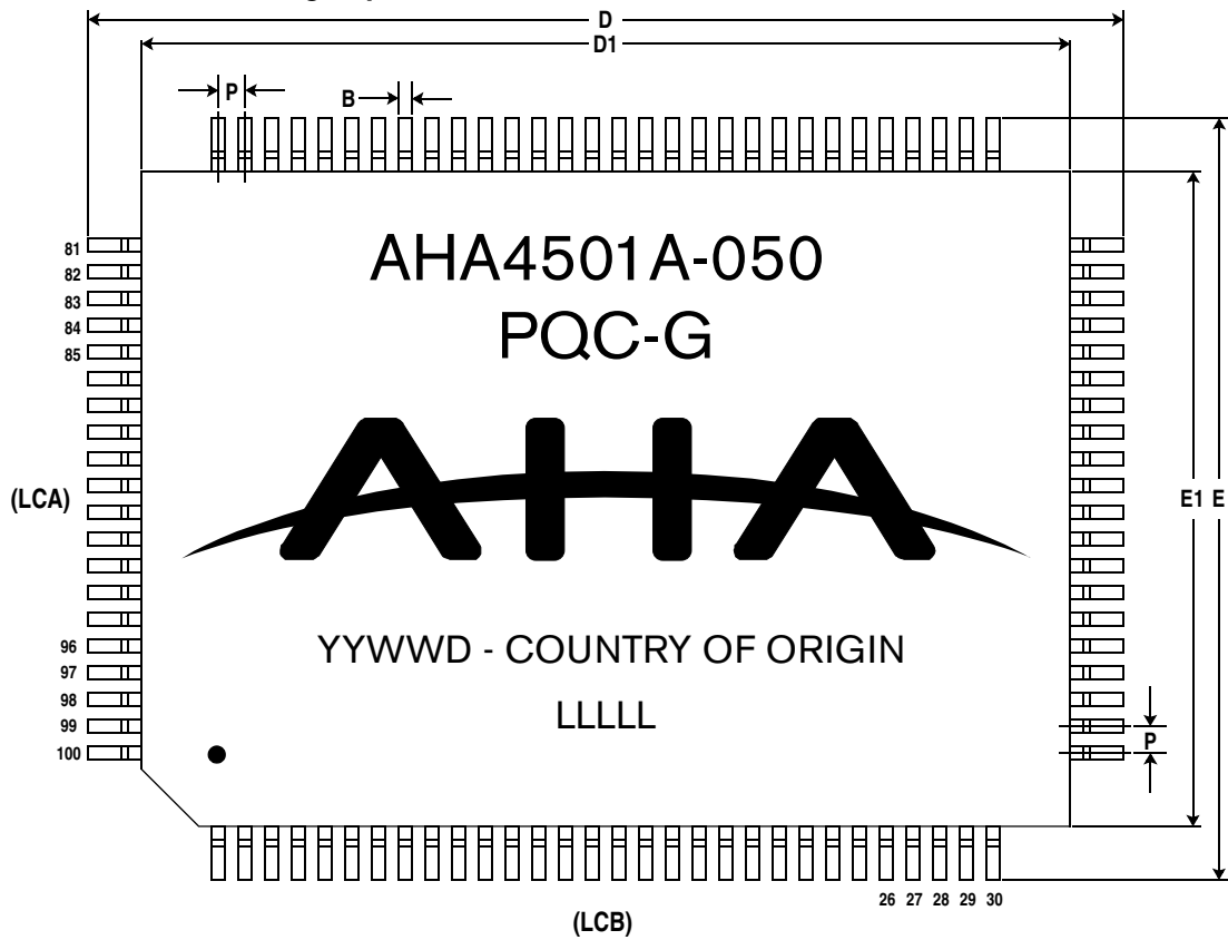
Figure 29: AHA4501 Package Specifications – 100 MQFP
