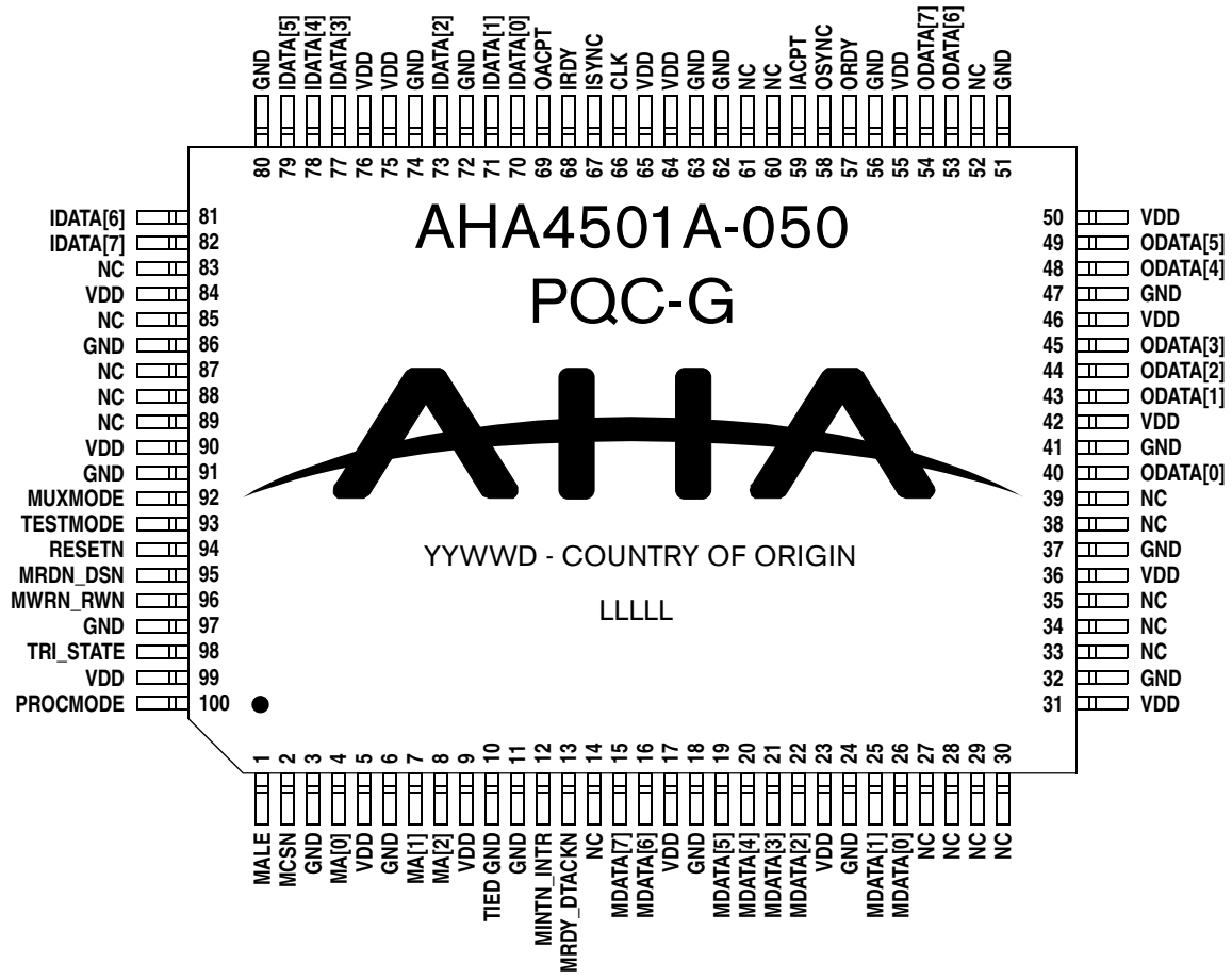
Figure 15: Pinout – 100 MQFP
