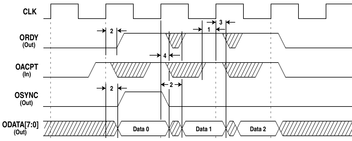
Figure 19: Data Output Timing
