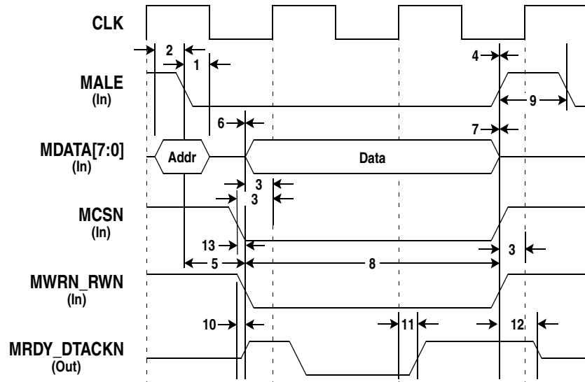
Figure 22: Microprocessor Interface Timing (Write); PROCMODE=0, MUXMODE=1
