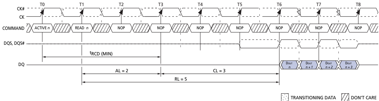
Figure 11: READ Latency
