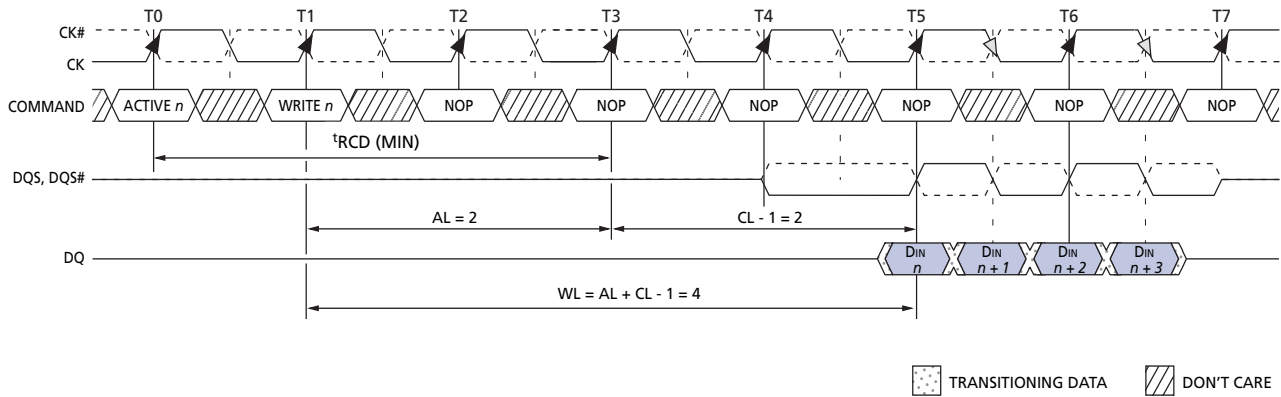
Figure 12: WRITE Latency
