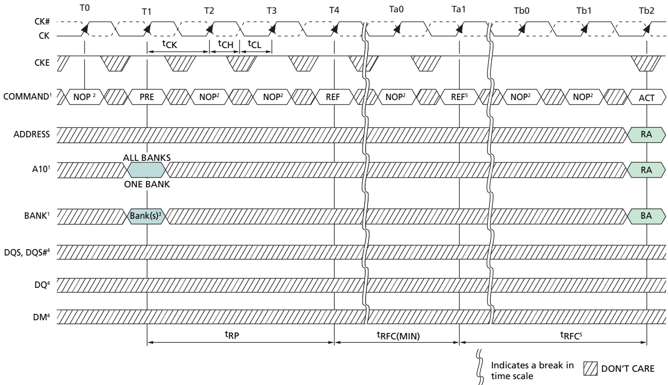
Figure 44: Refresh Mode
