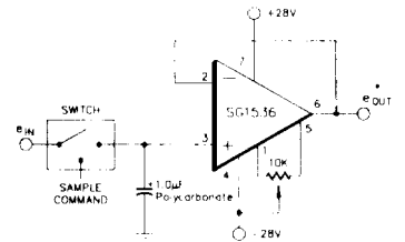
FIGURE 8 - LOW-DRIFT SAMPLE AND HOLD
