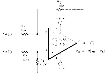
FIGURE 7 - DIFFERENTIAL AMPLIFIER WITH ±20V COMMON-MODE INPUT VOLTAGE RANGE
