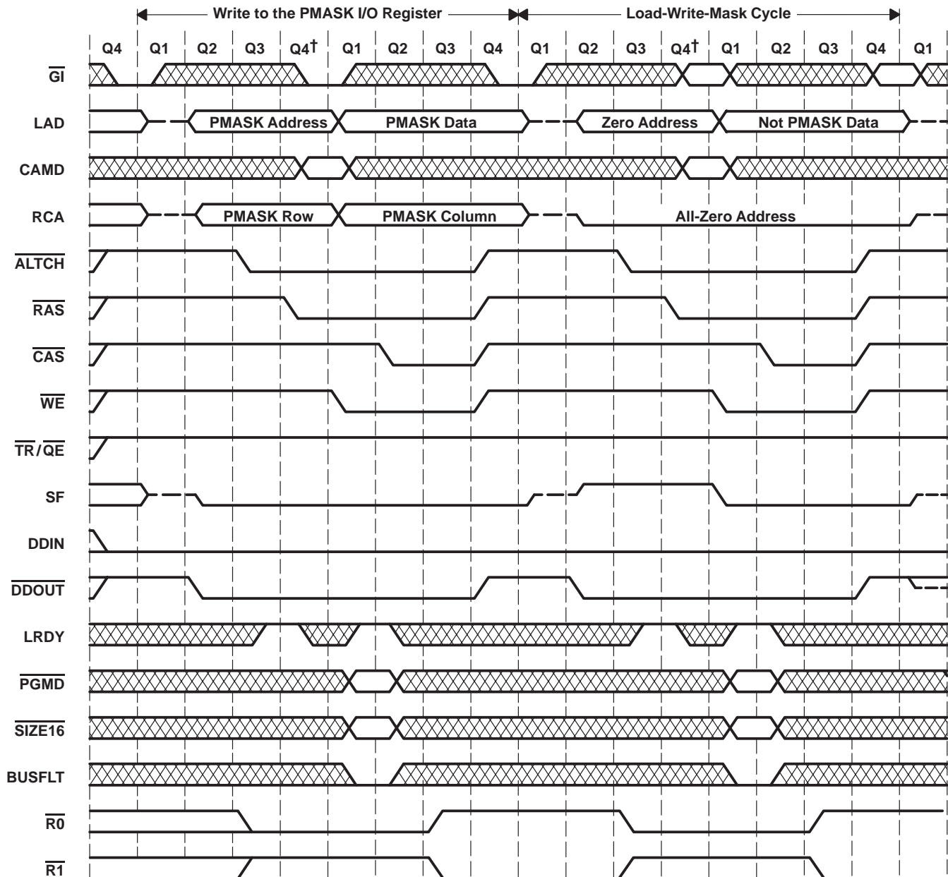
Figure 9. Load-Write-Mask-Cycle Timing
