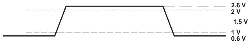
Figure 31. TTL-Level Outputs
