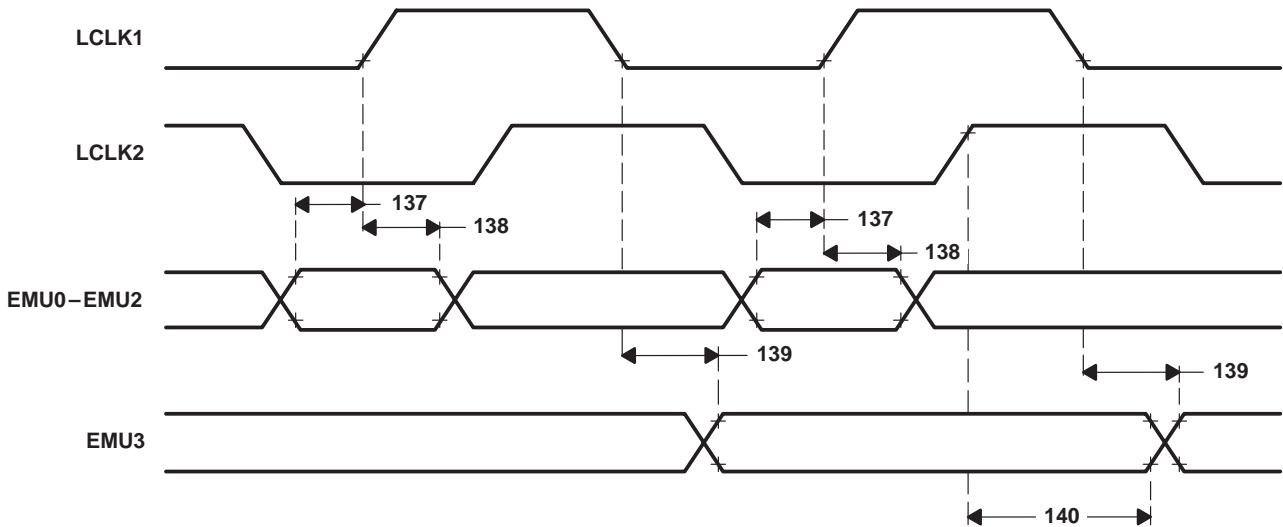
Figure 51. Emulator-Interface Timing
