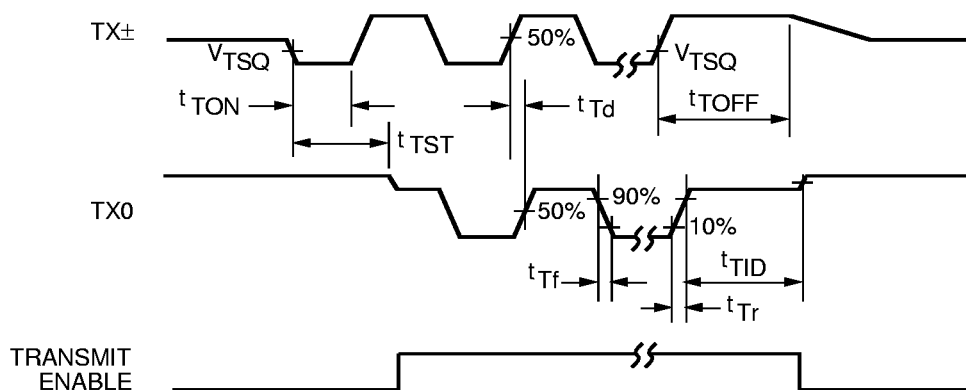
Figure 3. Transmitter Timing
