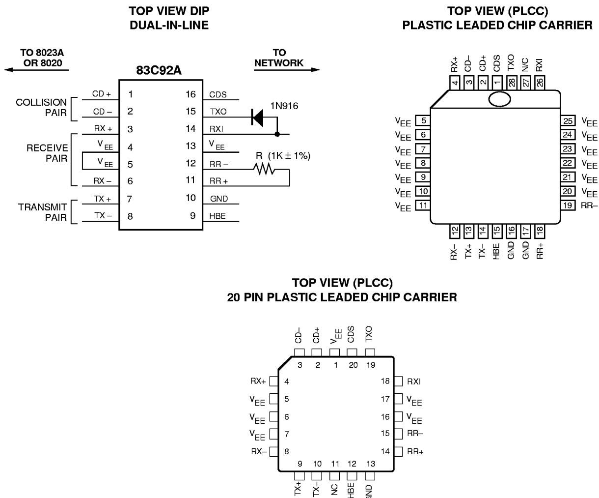
Figure 2. 83C92A Ethernet Transceiver Pin Configuration
