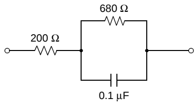
Figure 15. Termination Impedance
