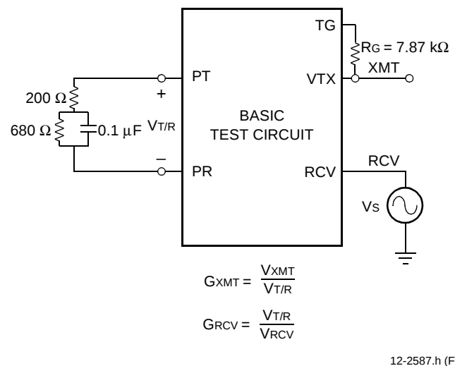
Figure 11. ac Gains
