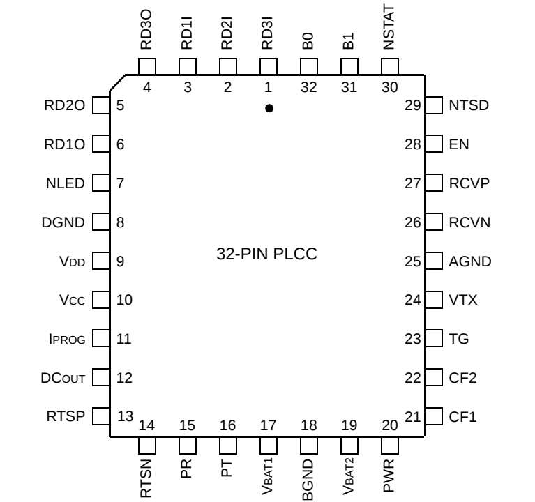
Figure 2. 32-Pin Diagram (PLCC Chip)
