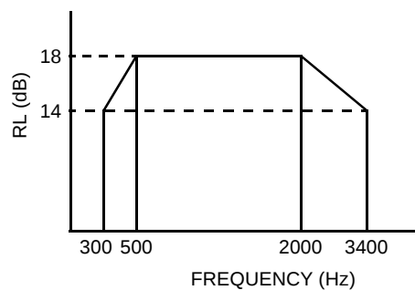
Figure 18. Return Loss
