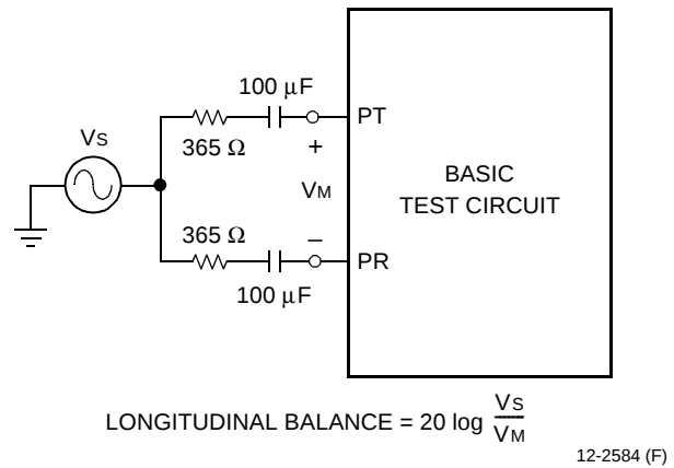
Figure 9. Longitudinal Balance
