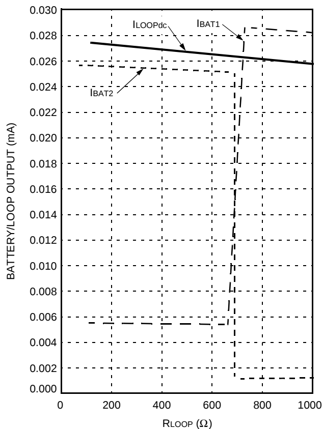
Figure 24. L8567 Loop/Battery Current (with Battery Switch) vs. Loop Resistance
