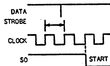
Fig. 1 UAR/T - TRANSMITTER TIMING
