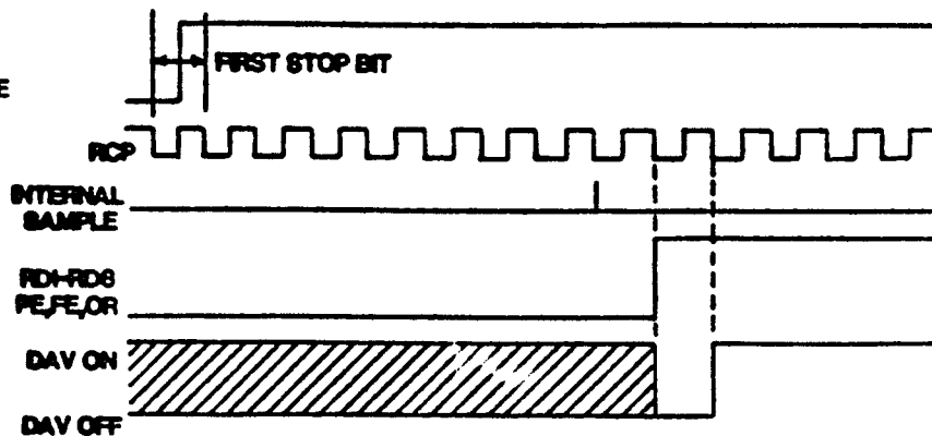
Fig. 6 UAR/T - RECEIVER TIMING
