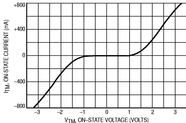
Figure 2. On-State Characteristics
