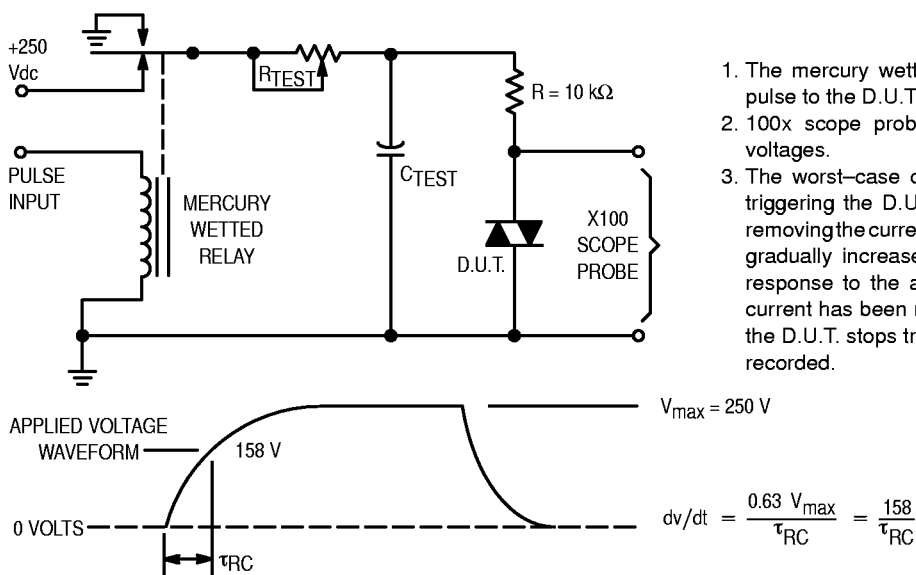
Figure 6. Static dv/dt Test Circuit
