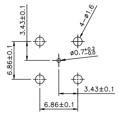
Recommended PC Board Layout Without Mounting Posts
