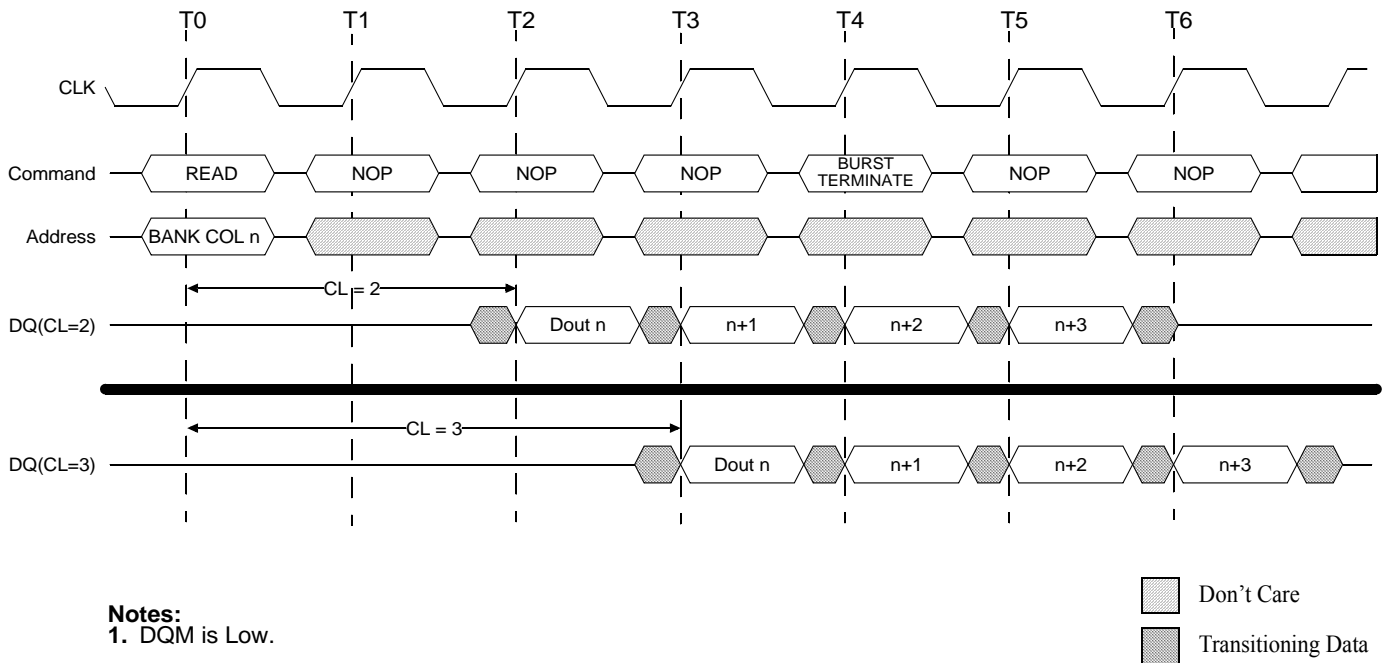
Figure 15: Terminating a READ Burst
