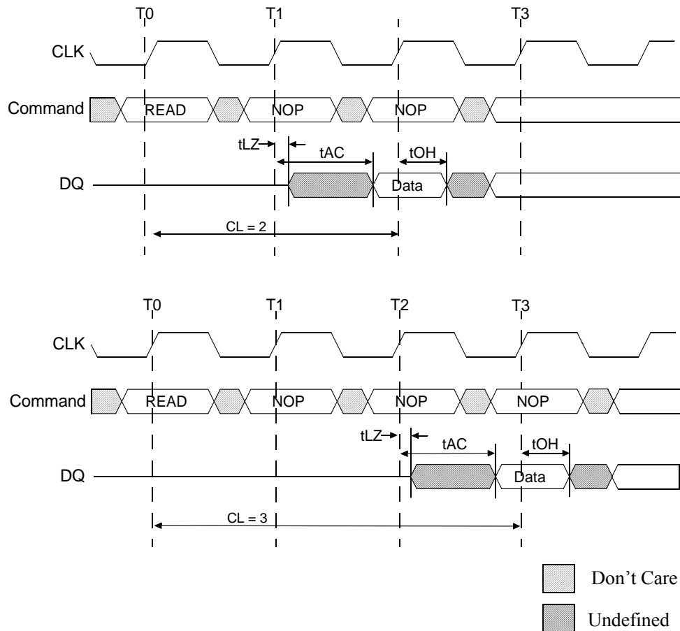
Figure 5: CAS Latency
