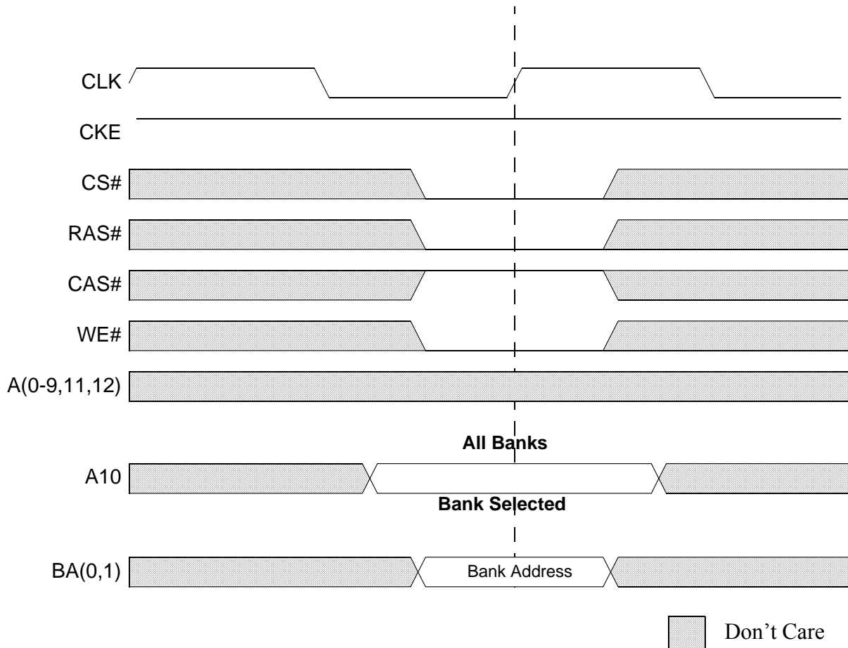
Figure 23: PRECHARGE Command
