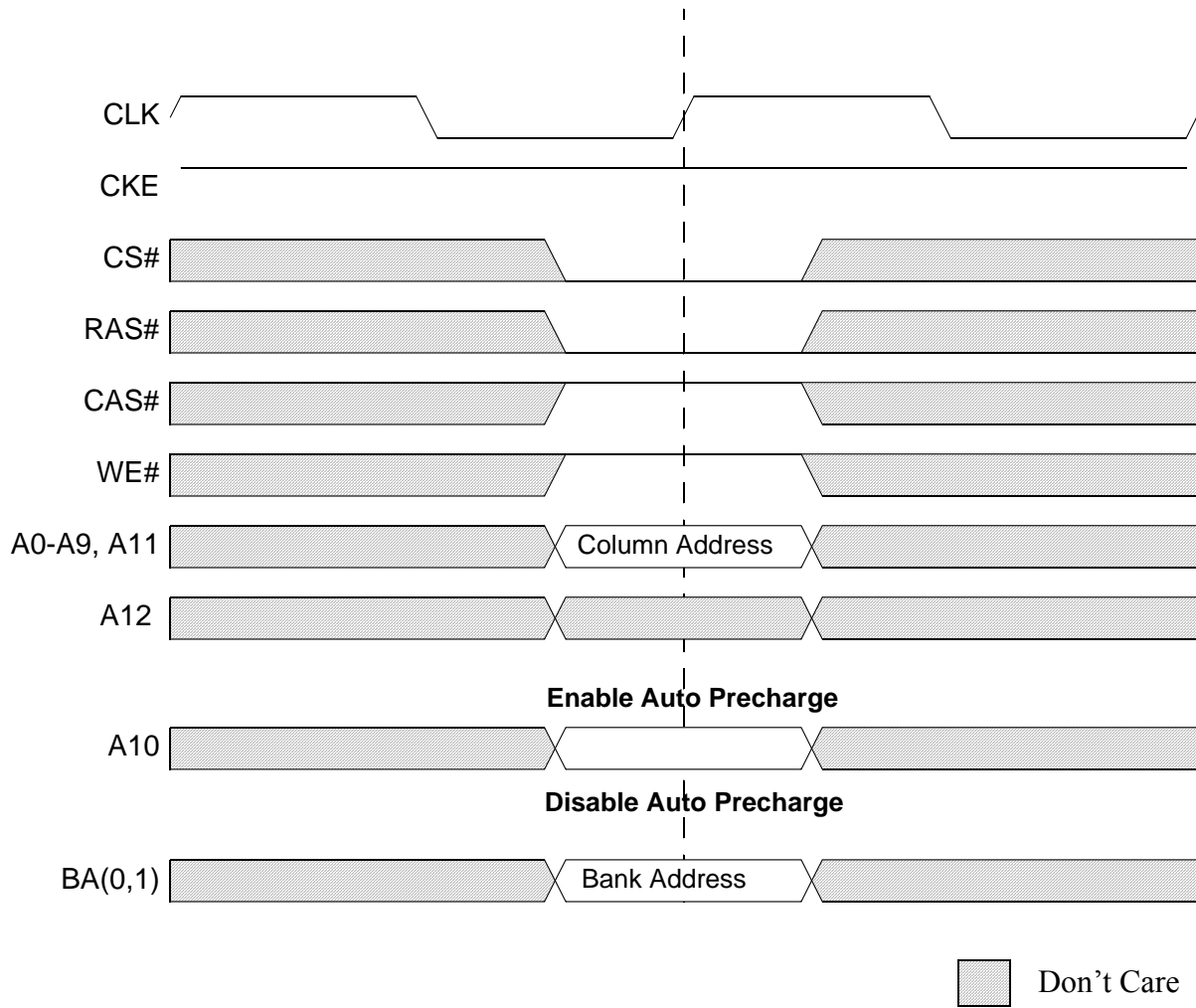
Figure 8: READ Command
