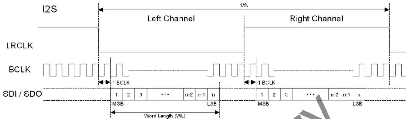
Figure 13. I 2 S Justified Audio Interface (assuming n-bit word length)
