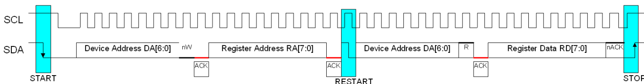
Figure 17. Read Cycle
