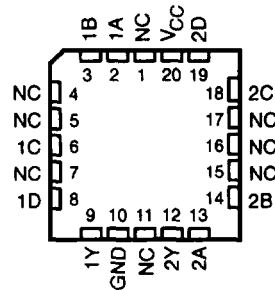
SN54ALS21A, SN54AS21 ... FK PACKAGE (TOP VIEW)
