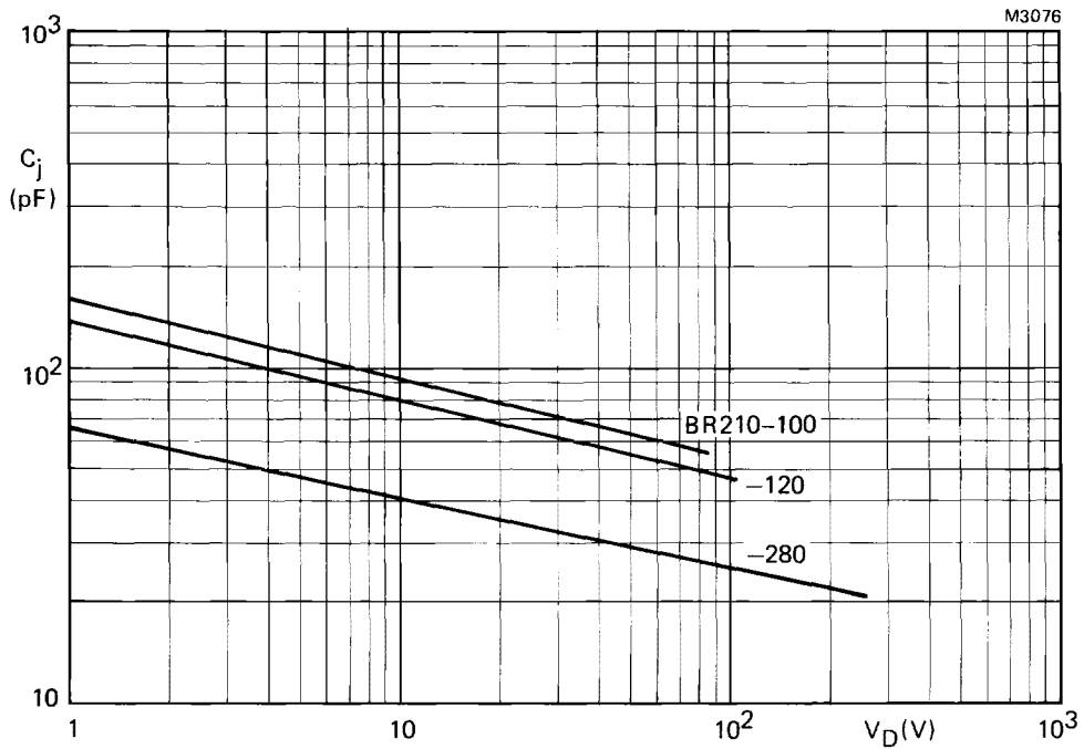
Fig. 14 Typical junction capacitance as a function of off-state voltage; T_j = 25^\circ\text{C} ; f = 1\text{ MHz} .
