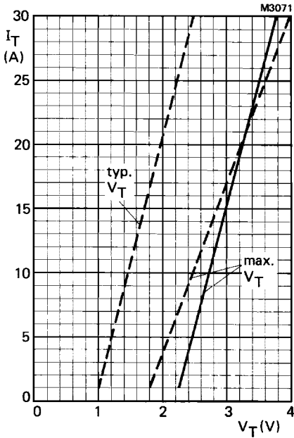
Fig.9 On-state voltage as a function of on-state current. (200 \mu\text{s} pulsed condition to avoid excessive dissipation) — T_j = 25^\circ\text{C} , - - - T_j = 125^\circ\text{C} .
