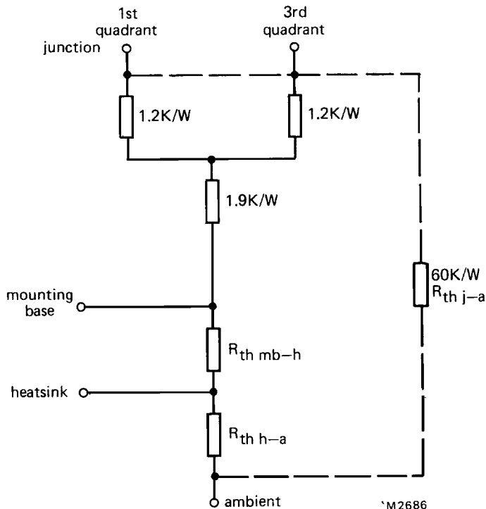
Fig.2 Components of thermal resistance (junction to ambient).
