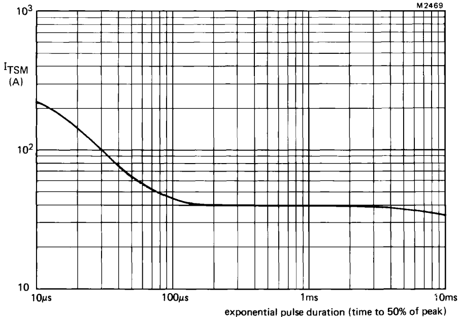
Fig.8 Maximum non-repetitive exponential waveform Impulse Current rating as a function of pulse duration (virtual front-time 10\ \mu\text{s} ).
