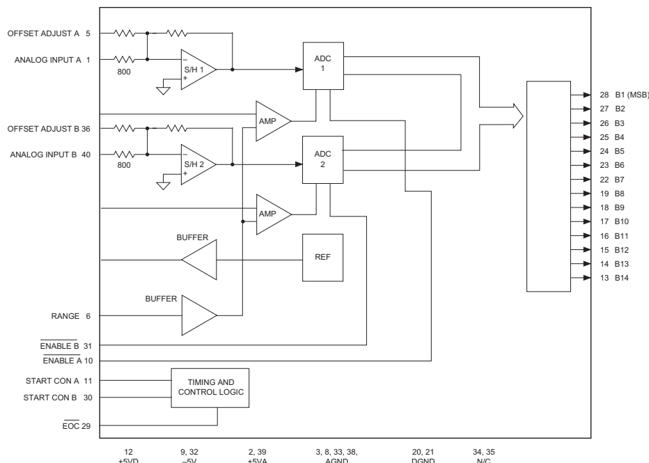
Figure 1. ADSD-1402 Functional Block Diagram
