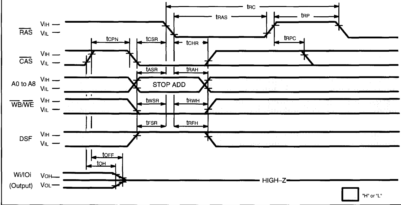
Fig. 19 – \overline{\text{CAS}} -BEFORE- \overline{\text{RAS}} REFRESH CYCLE (STOP REGISTER SET) ( \overline{\text{DT}}/\overline{\text{OE}} and W0/IO0 to W7/IO7 (input) = "H" or "L")
