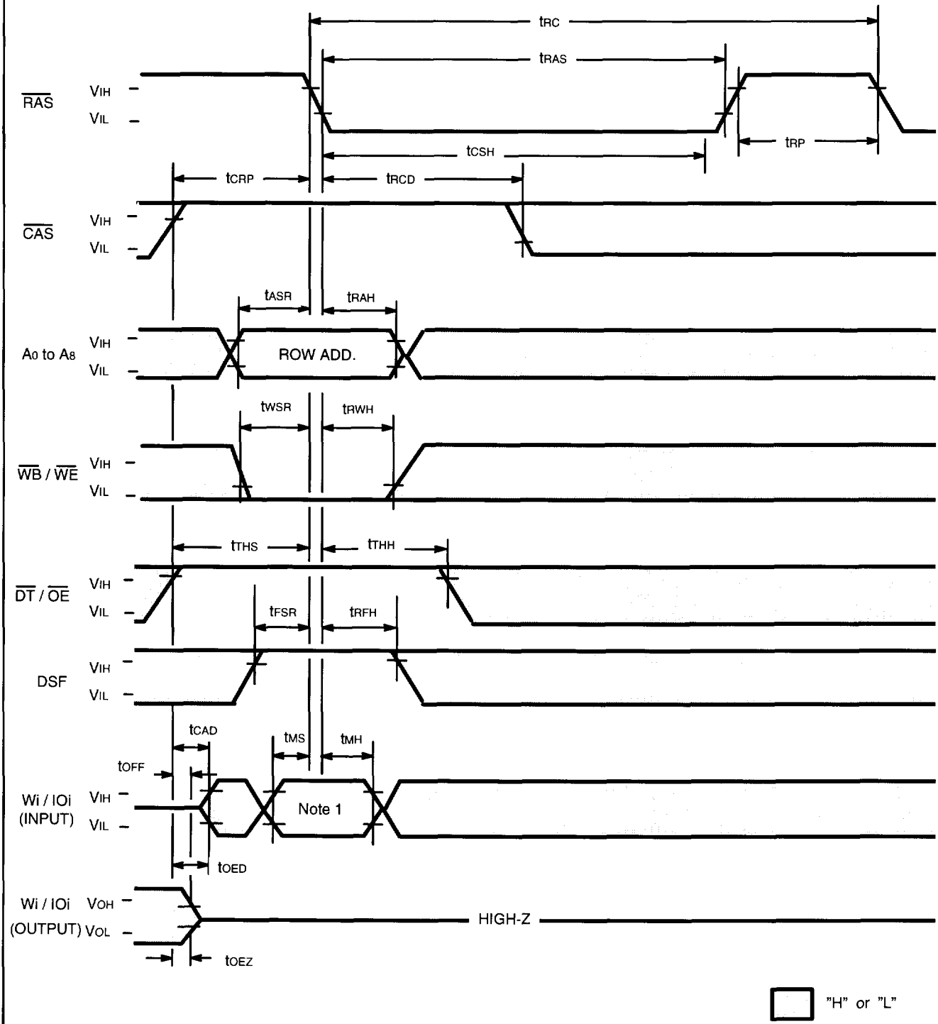
Fig. 22 – FLASH WRITE CYCLE
