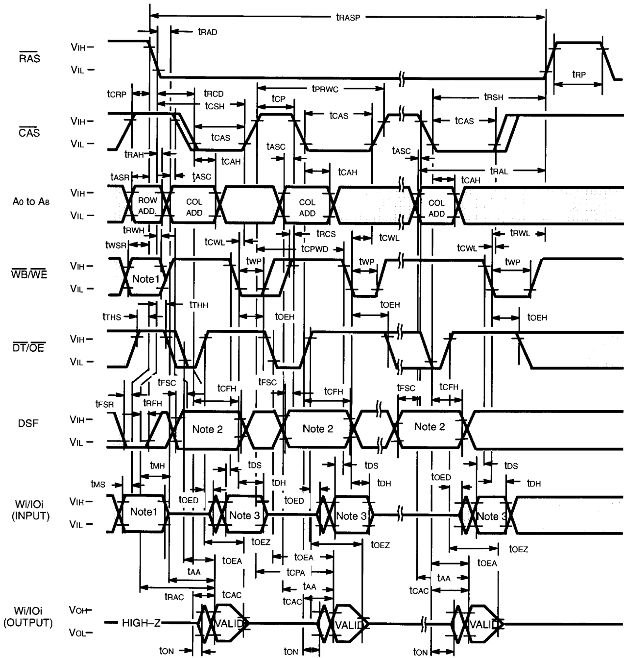
Fig. 16 – FAST PAGE MODE READ-MODIFY-WRITE CYCLE
