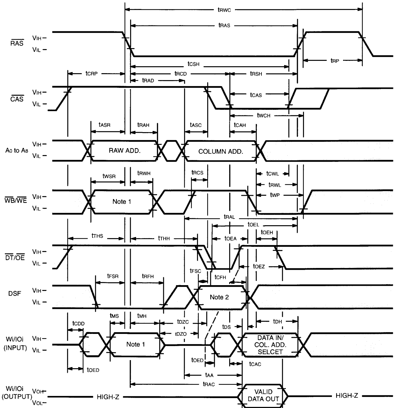
Fig. 12 – READ•WRITE/READ-MODIFY-WRITE CYCLE
