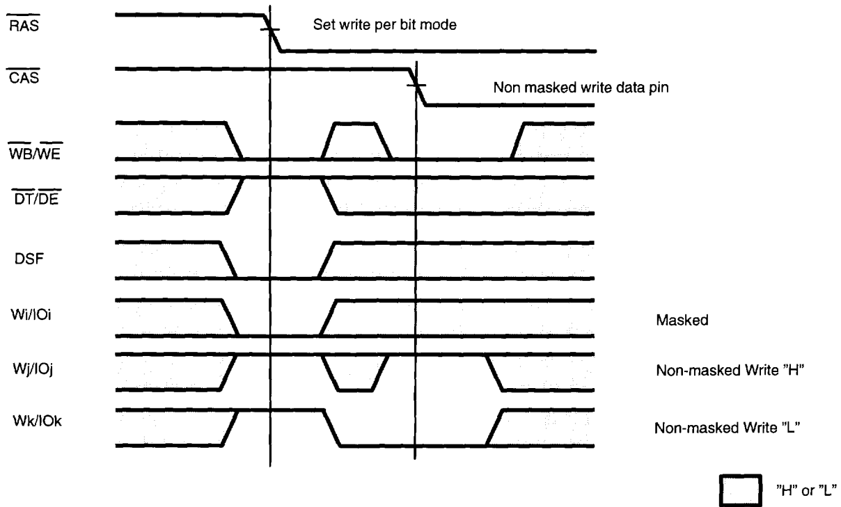
Fig. 2 - EXAMPLE OF WRITE-PER-BIT OPERATION FOR NEW MASK
