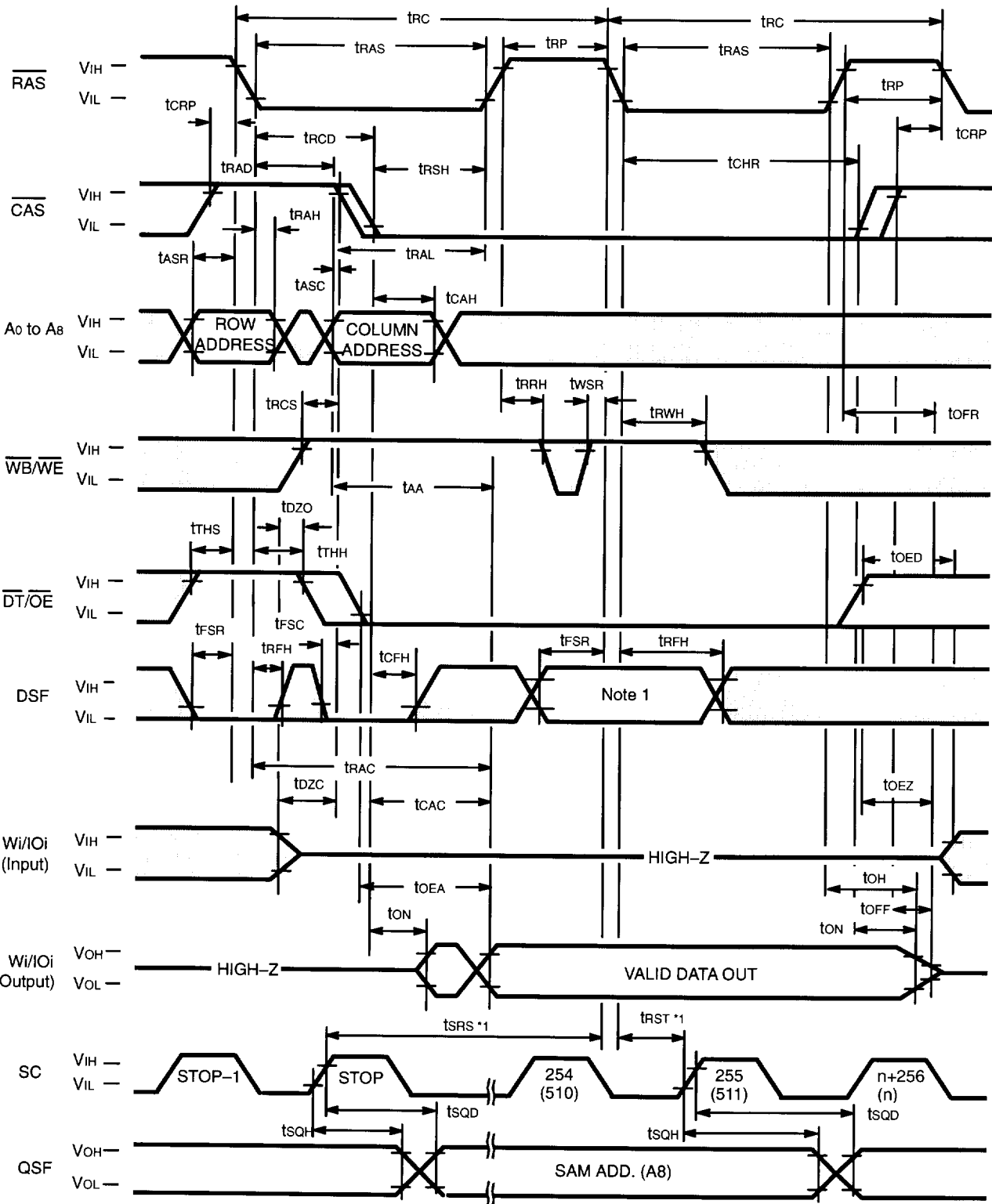
Fig. 21 - HIDDEN REFRESH CYCLE
