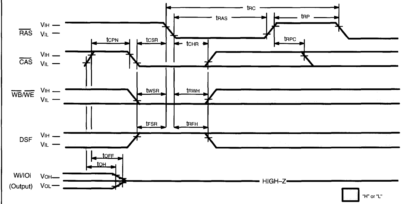
Fig. 20 – \overline{\text{CAS}} -BEFORE- \overline{\text{RAS}} REFRESH CYCLE (OPTION NO-RESET) (A0 to A8, \overline{\text{DT}}/\overline{\text{OE}} and W0/IO0 to W7/IO7 (input) = "H" or "L")
