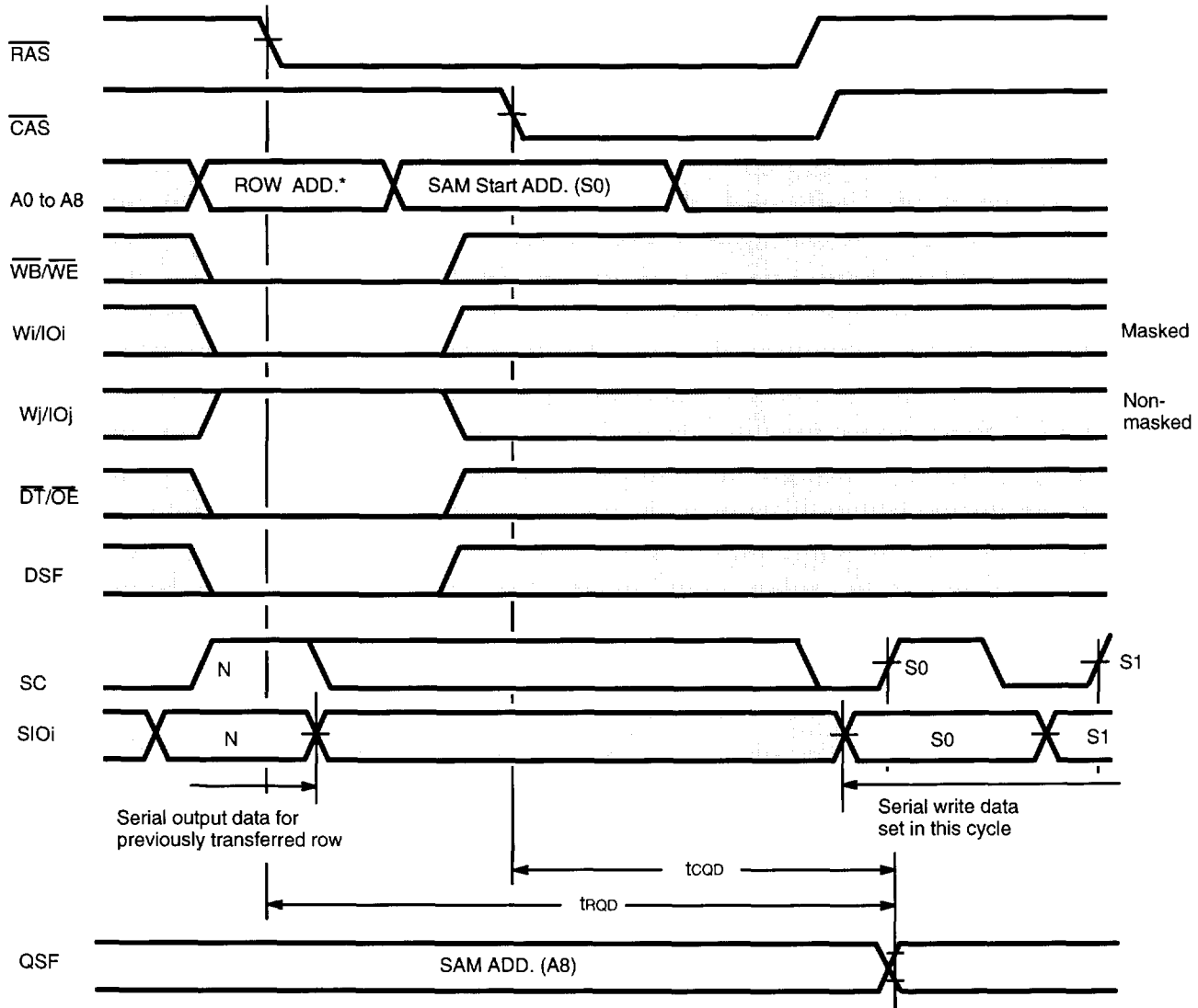
Fig. 4 - EXAMPLE OF WRITE TRANSFER CYCLE FOR NEW MASK
