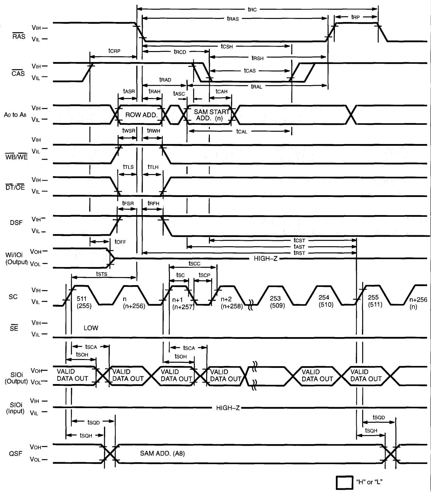
Fig. 31 - SPLIT READ TRANSFER CYCLE
