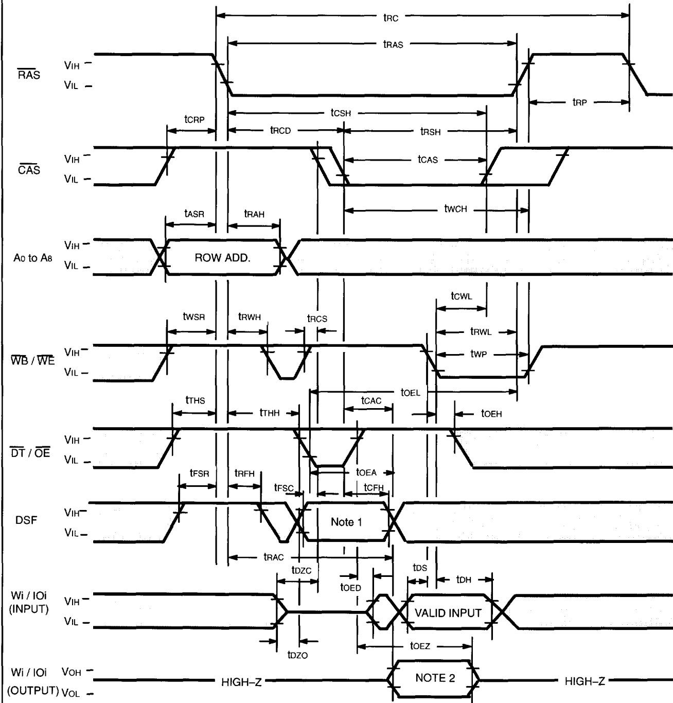
Fig. 25 – LOAD REGISTER CYCLE ( \overline{OE} CONTROL)
