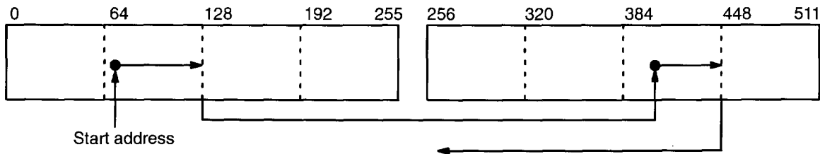
After boundary final address is accessed, SAM address jumped to initial address in the opposite SAM.
