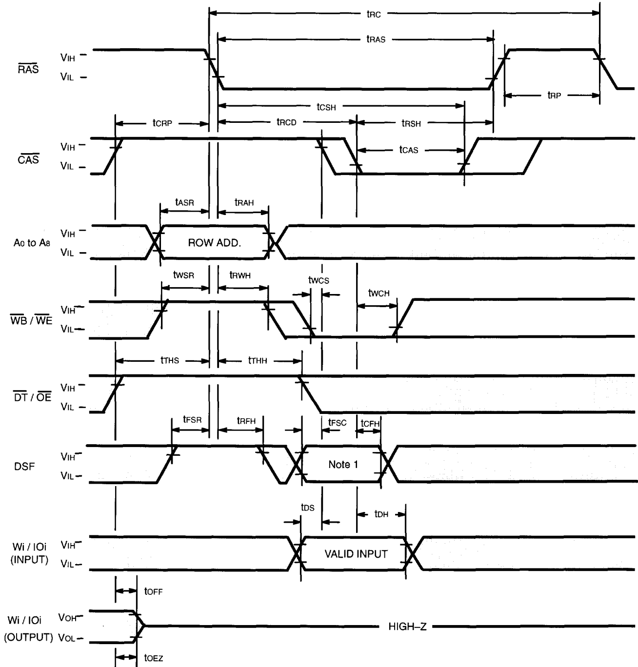
Fig. 24 - LOAD REGISTER CYCLE (EARLY WRITE)
