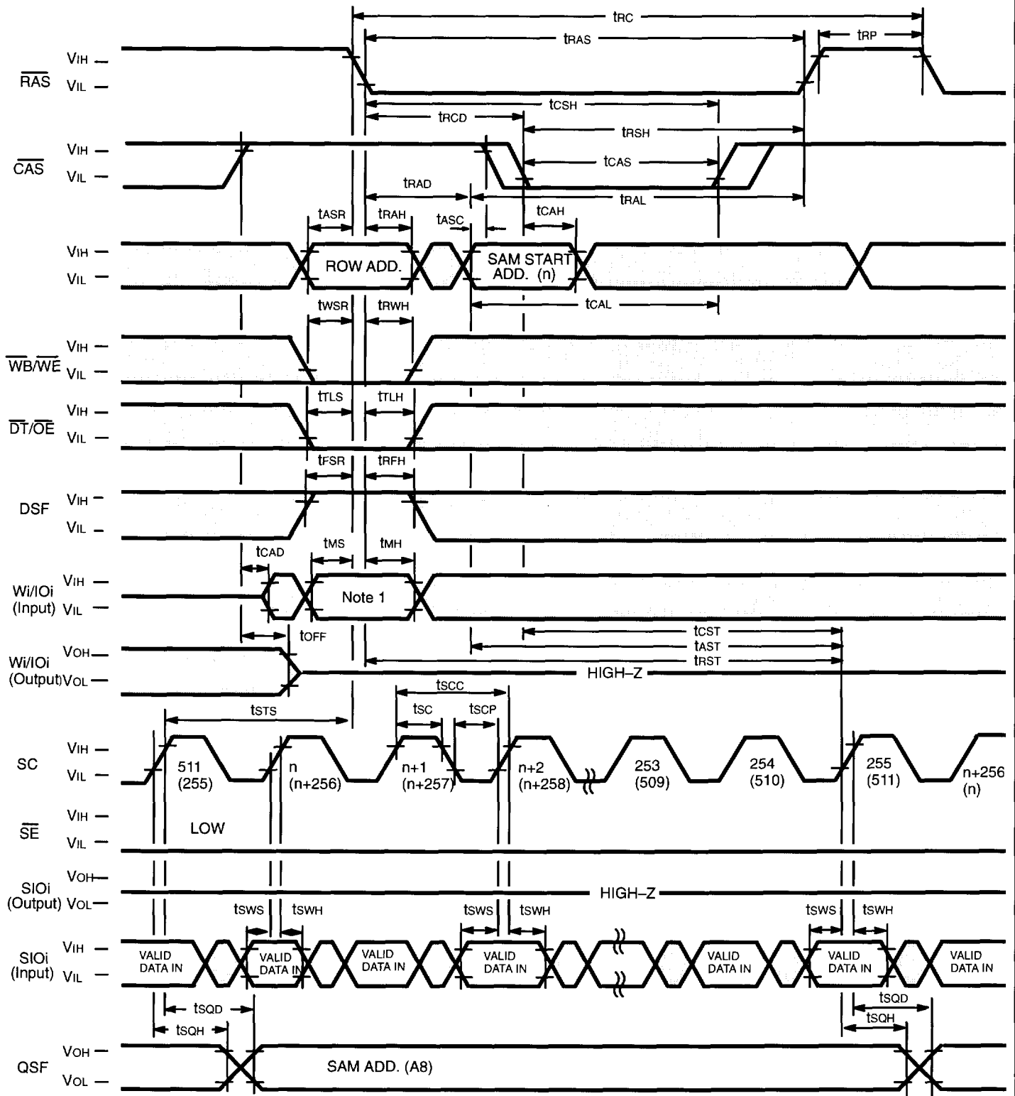
Fig. 32 – MASKED SPLIT WRITE TRANSFER CYCLE
