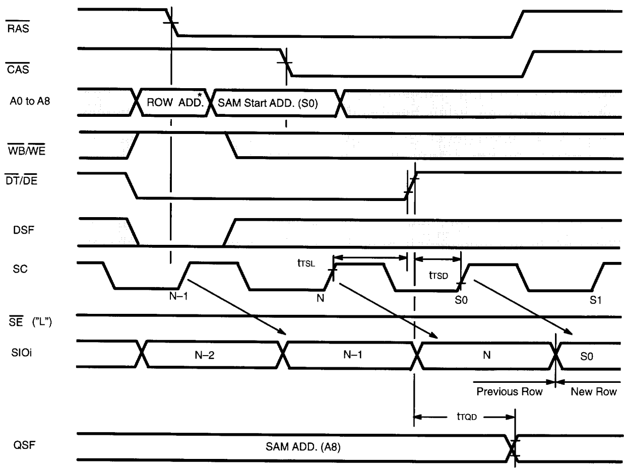
Fig. 3 - EXAMPLE OF REAL TIME READ TRANSFER OPERATION
