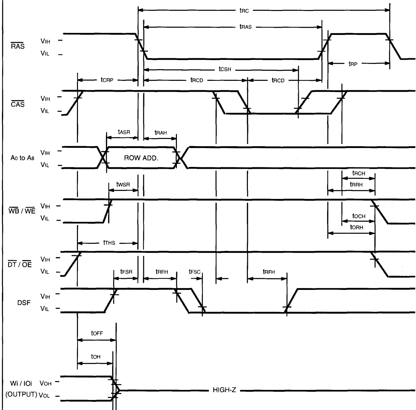
Fig. 26 - OLD MASK MODE RESET CYCLE
