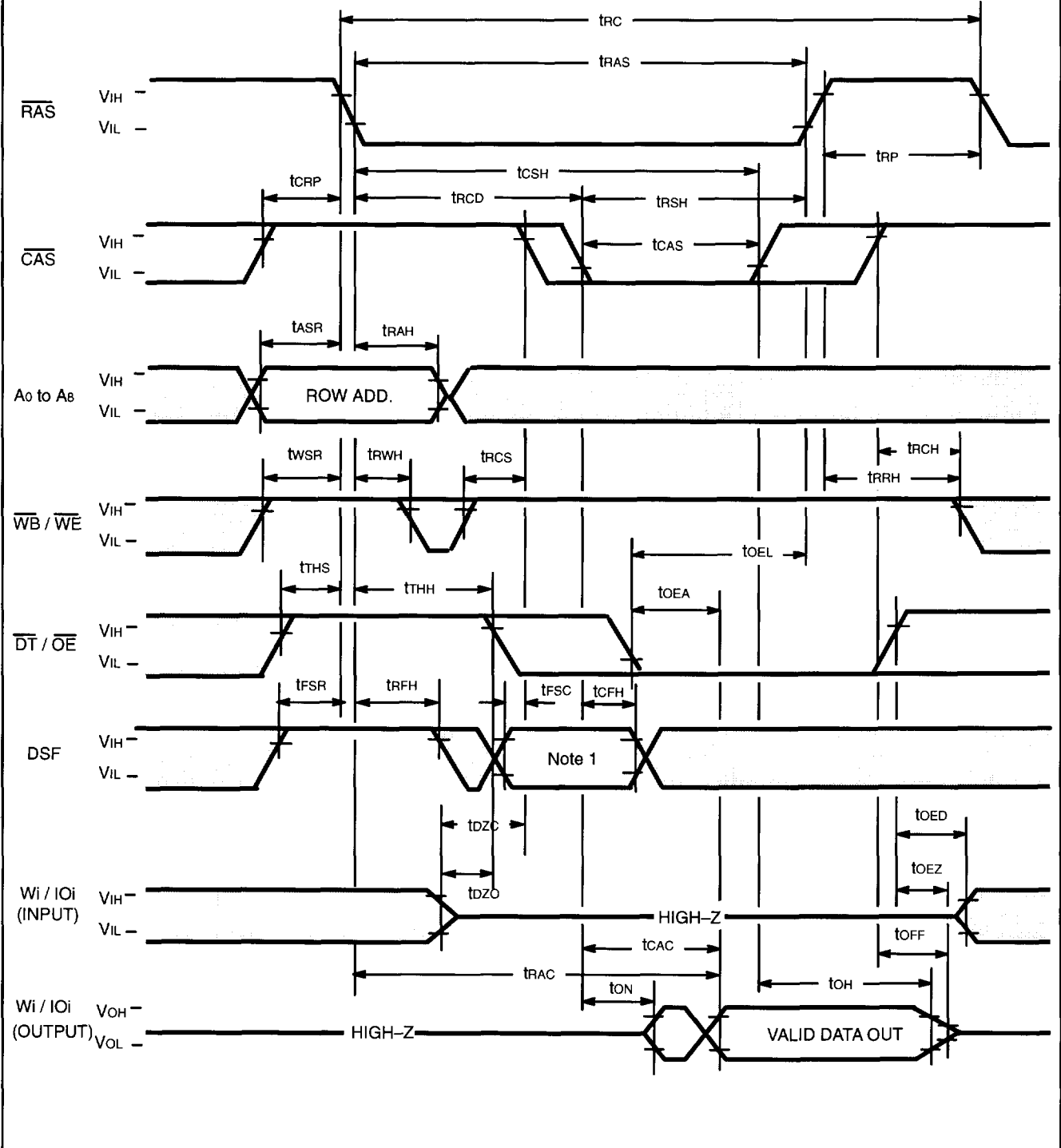
Fig. 23 - REGISTER READ CYCLE
