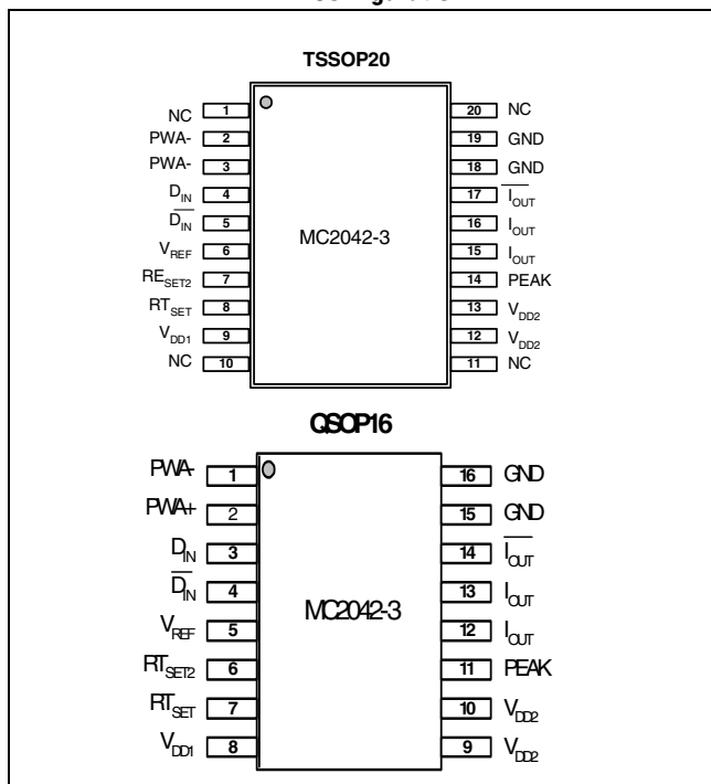
Pin Configuration
