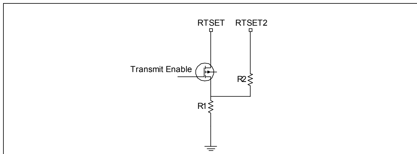
Figure 3-2. Transmit Enable/Disable
