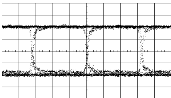
Fig.7 PECL RX data output NRZI mode
