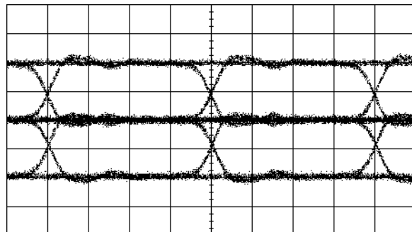
Fig.6 Transmit output MLT-3 data
