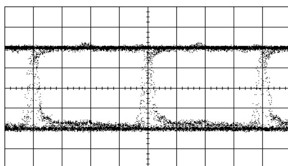
Fig.8 PECL RX data output MLT-3 mode
