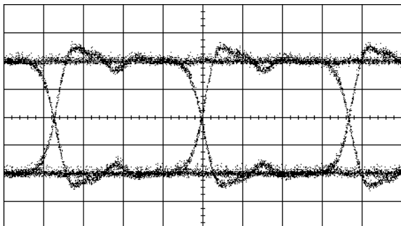
Fig.5 Transmit output NRZI data
