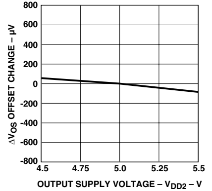
Figure 5. Input Offset Voltage Change vs. V_{DD2} .
