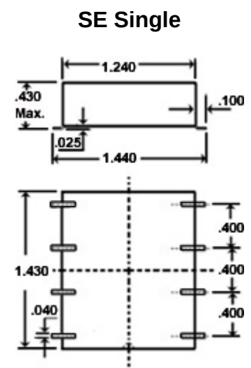
BOTTOM VIEW
